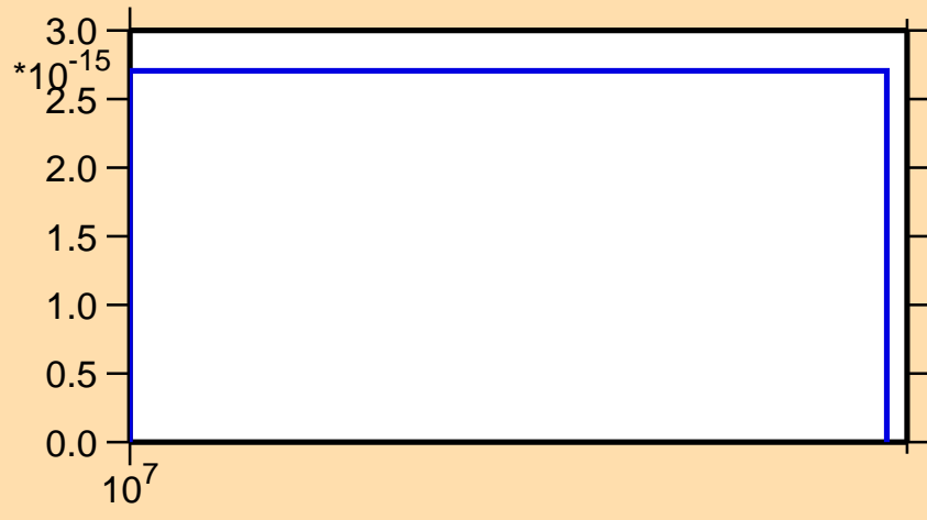
\sigma vs. E for ^{194}\text{Pt}(n,3n\alpha)
