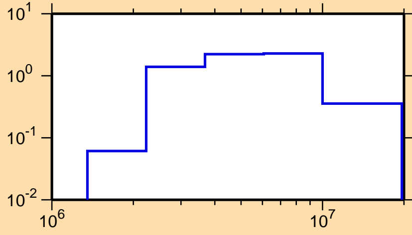
\sigma vs. E for ^{194}\text{Pt}(n,n\text{cont.})
