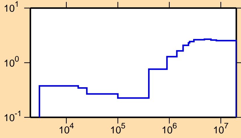
\sigma vs. E for ^{194}\text{Pt}(n,\text{nonel.})
