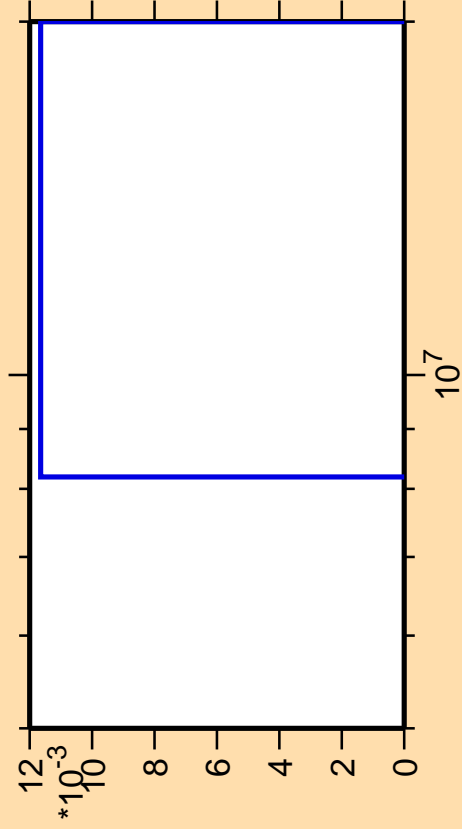
\Delta\sigma/\sigma vs. E for ^{194}\text{Pt}(n,3n\alpha)
