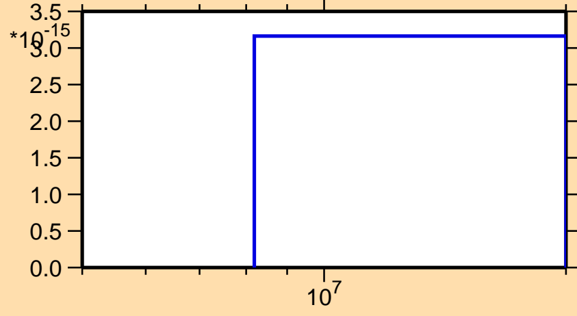
\sigma vs. E for ^{194}\text{Pt}(n,3n\alpha)
