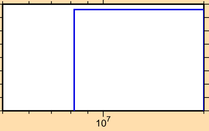
\sigma vs. E for ^{194}\text{Pt}(n,3n)
