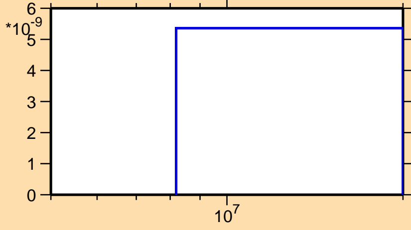
\sigma vs. E for ^{194}\text{Pt}(n,2n\alpha)
