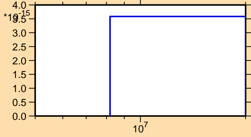
\sigma vs. E for ^{194}\text{Pt}(n,p\alpha)
