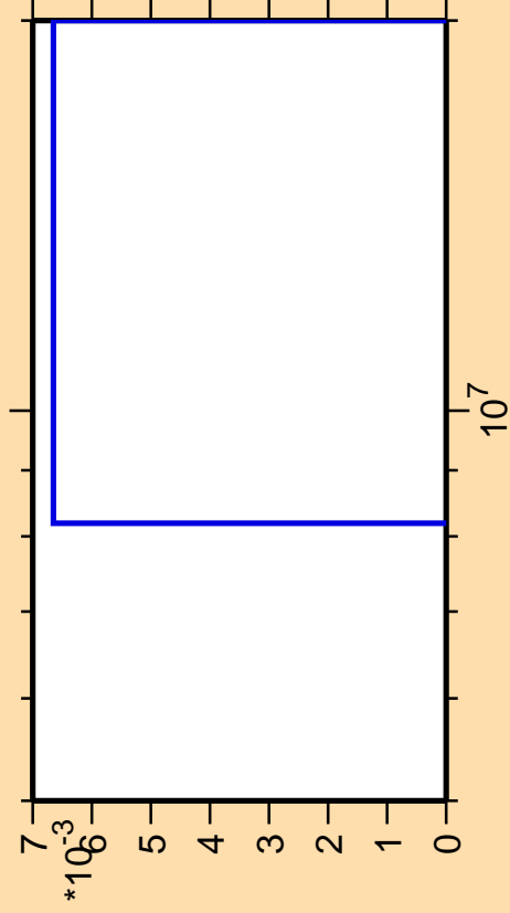
\Delta\sigma/\sigma vs. E for ^{194}\text{Pt}(n,p\alpha)
