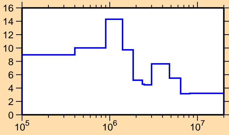
\Delta\sigma/\sigma vs. E for ^{194}\text{Pt}(n,\text{tot.})
