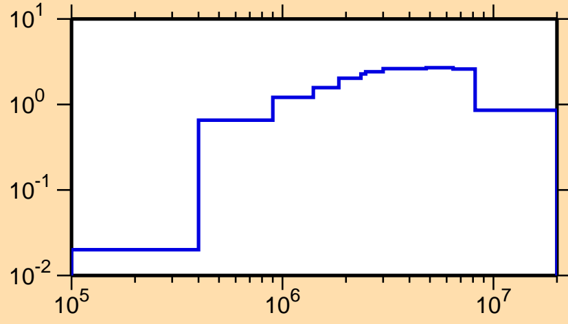
\sigma vs. E for ^{194}\text{Pt}(n,\text{inel.})
