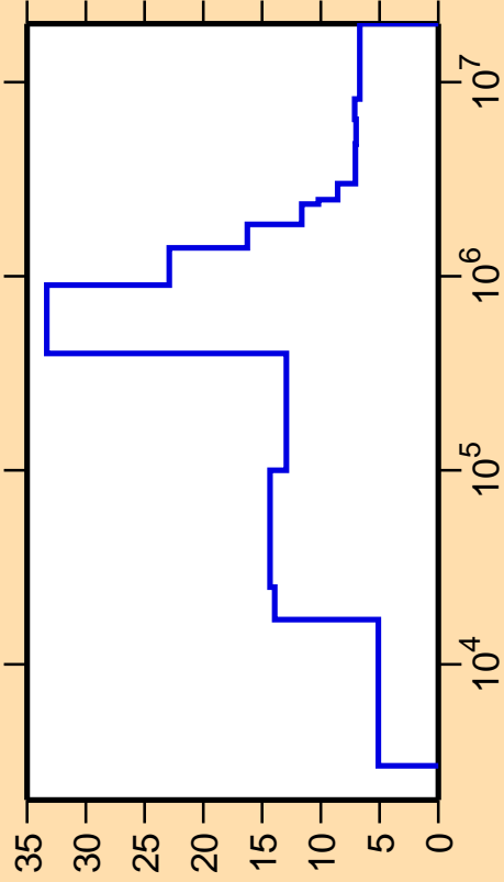
\Delta\sigma/\sigma vs. E for ^{194}\text{Pt}(n,\text{nonel.})
