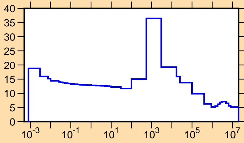
\sigma vs. E for ^{194}\text{Pt}(n,\text{tot.})
