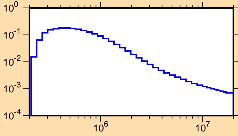
\sigma vs. E for ^{195}\text{Pt}(n,n_4)
