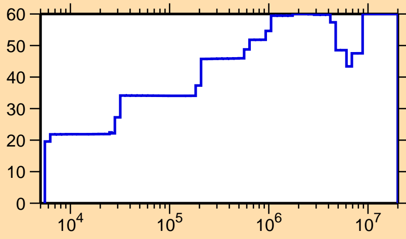
\Delta\sigma/\sigma vs. E for ^{195}\text{Pt}(n,\gamma)
