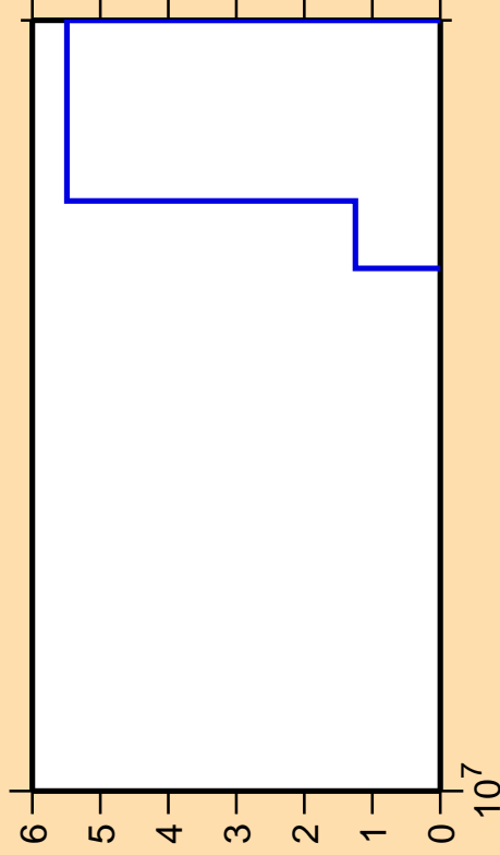
\Delta\sigma/\sigma vs. E for ^{195}\text{Pt}(n,p\alpha)
