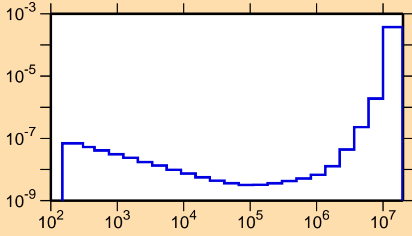
\sigma vs. E for ^{195}\text{Pt}(n,\alpha)
