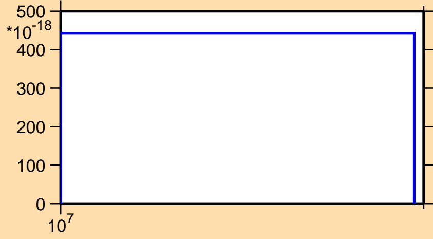
\sigma vs. E for ^{195}\text{Pt}(n,3n\alpha)
