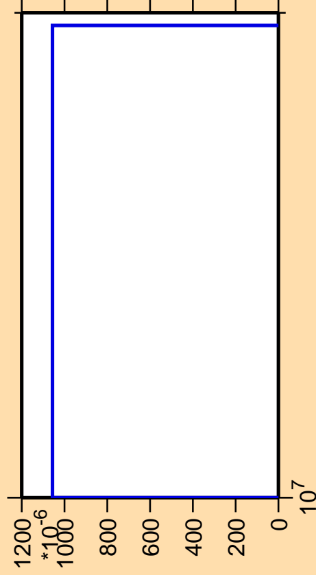
\Delta\sigma/\sigma vs. E for ^{195}\text{Pt}(n,3n\alpha)
