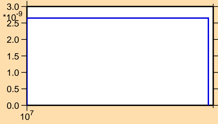
\sigma vs. E for ^{195}\text{Pt}(n,\text{nd})
