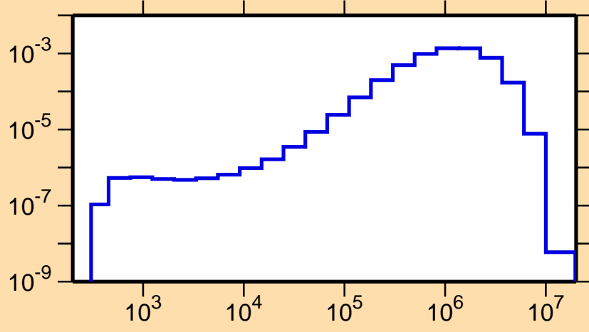
\sigma vs. E for ^{195}\text{Pt}(n,n_2)
