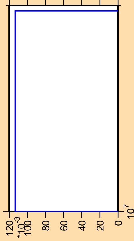
\Delta\sigma/\sigma vs. E for ^{195}\text{Pt}(n,p\alpha)
