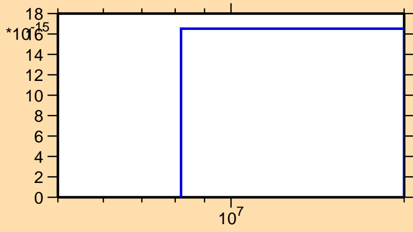
\sigma vs. E for ^{195}\text{Pt}(n,p\alpha)
