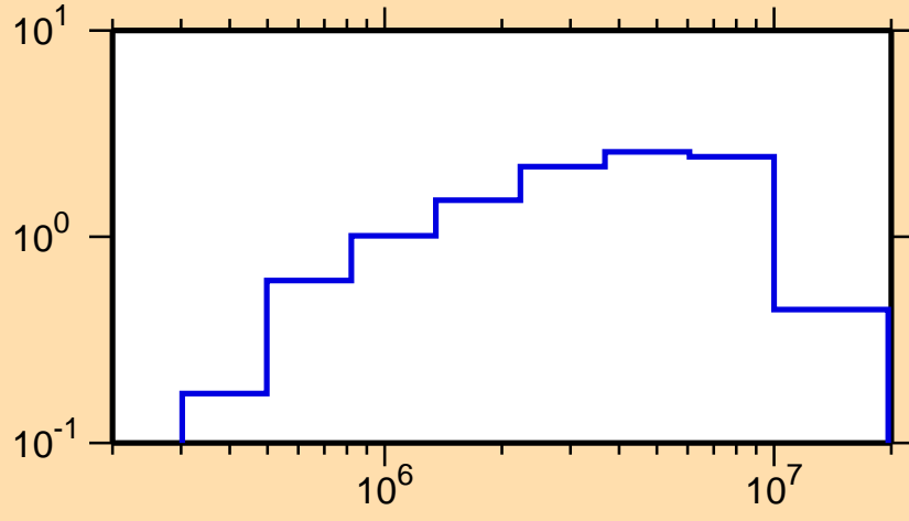
\sigma vs. E for ^{196}\text{Pt}(n,\text{inel.})
