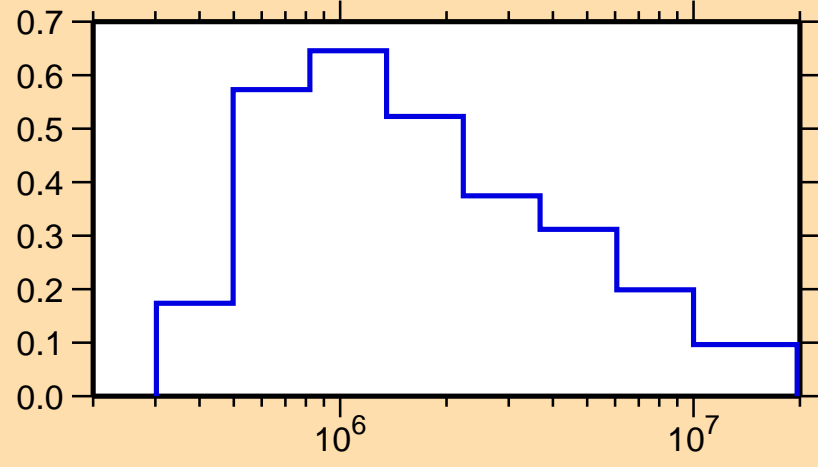
\sigma vs. E for ^{196}\text{Pt}(n,n_1)
