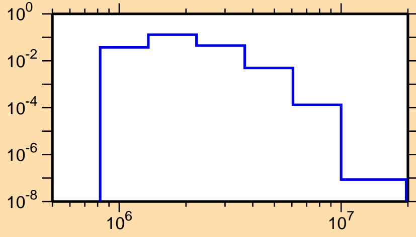
\sigma vs. E for ^{196}\text{Pt}(n,n_4)
