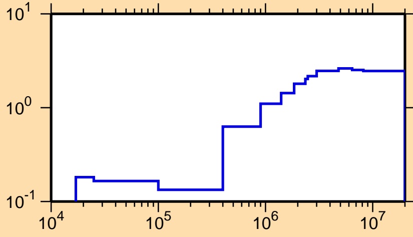
\sigma vs. E for ^{196}\text{Pt}(n,\text{nonel.})
