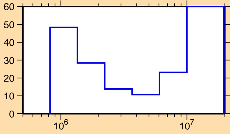
\Delta\sigma/\sigma vs. E for ^{197}\text{Pt}(n,n\text{cont.})
