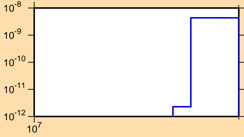
\sigma vs. E for ^{197}\text{Pt}(n,nt)
