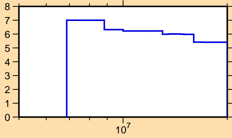
\Delta\sigma/\sigma vs. E for ^{198}\text{Pt}(n,\text{nonel.})
