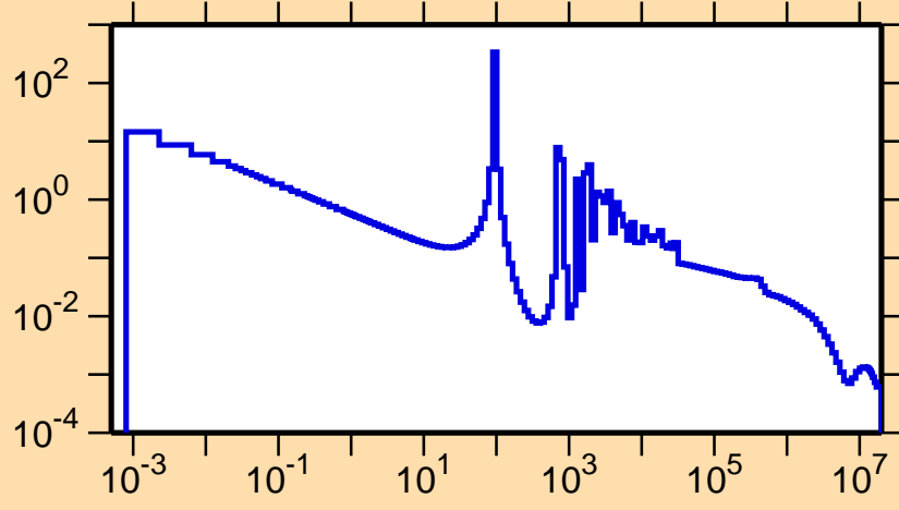
\sigma vs. E for ^{198}\text{Pt}(n,\gamma)
