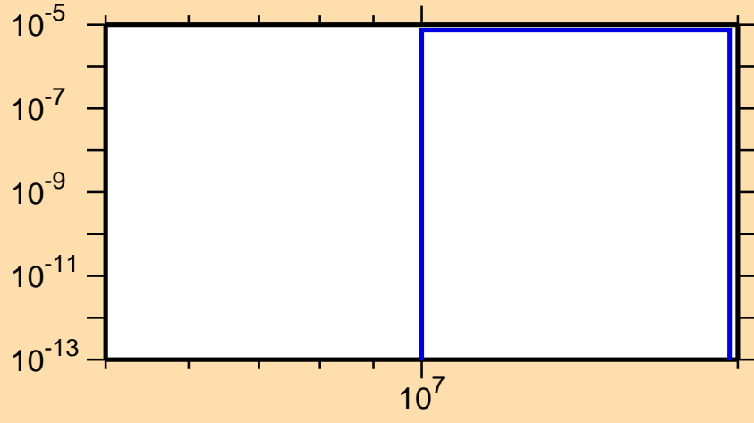
\sigma vs. E for ^{198}\text{Pt}(n,np)
