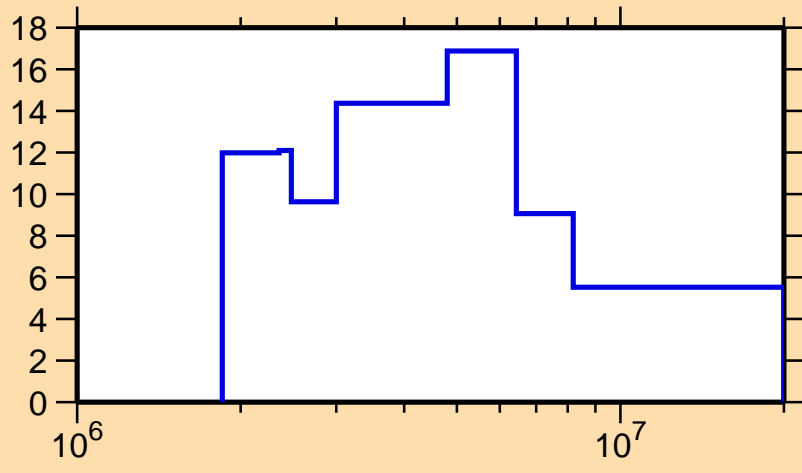
\Delta\sigma/\sigma vs. E for ^{198}\text{Pt}(n, el.)
