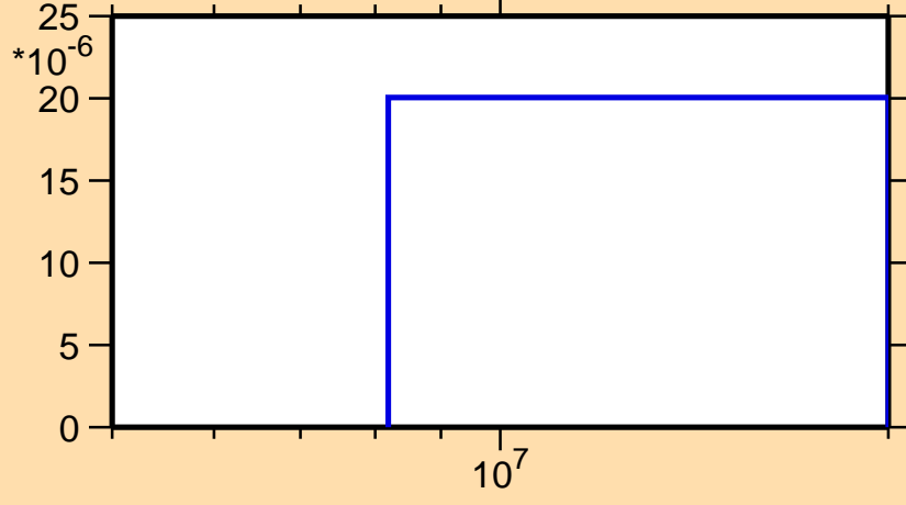
\sigma vs. E for ^{198}\text{Pt}(n,d)
