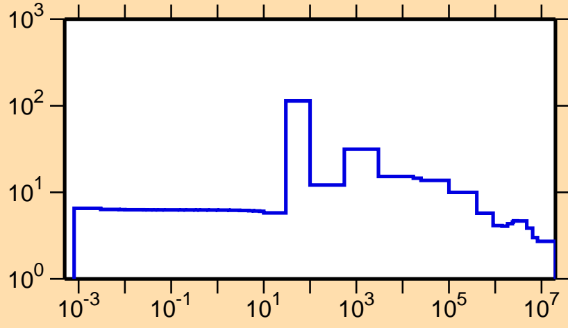
\sigma vs. E for ^{198}\text{Pt}(n,\text{el.})
