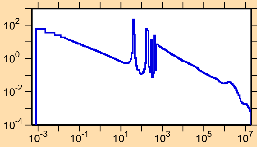
\sigma vs. E for ^{199}\text{Pt}(n,\gamma)
