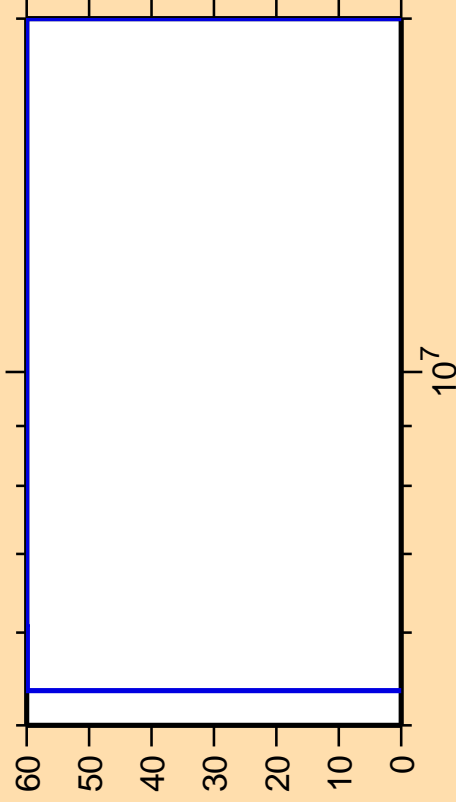
\Delta\sigma/\sigma vs. E for ^{199}\text{Pt}(n,n_1)
