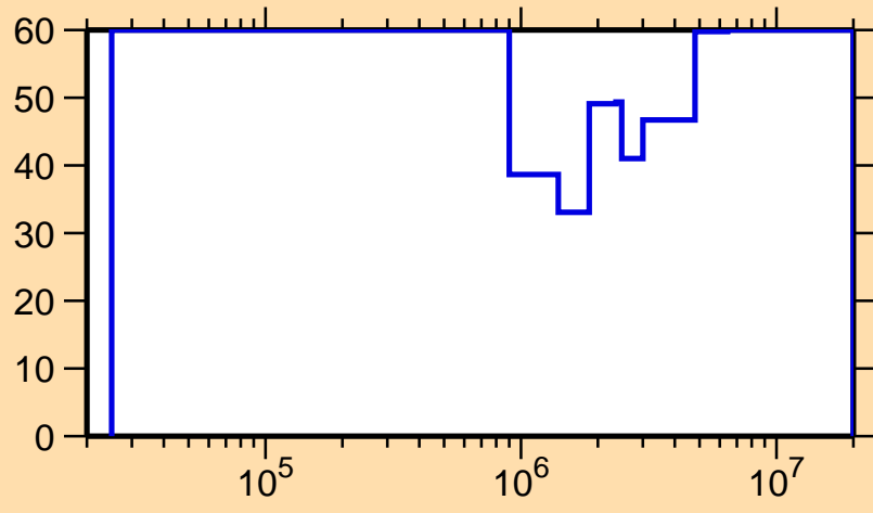
\Delta\sigma/\sigma vs. E for ^{199}\text{Pt}(n,n_1)
