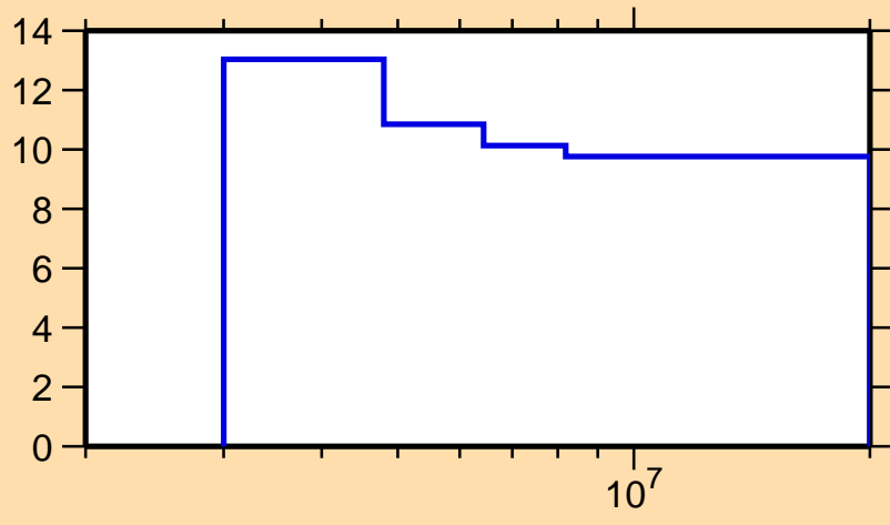
\Delta\sigma/\sigma vs. E for ^{199}\text{Pt}(n,\text{nonel.})
