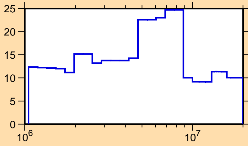
\Delta\sigma/\sigma vs. E for ^{199}\text{Pt}(n, el.)
