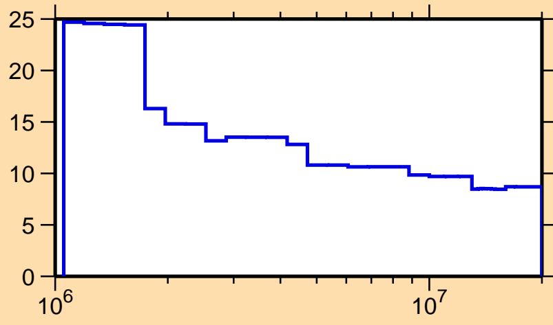
\Delta\sigma/\sigma vs. E for ^{199}\text{Pt}(n,n\text{onel.})
