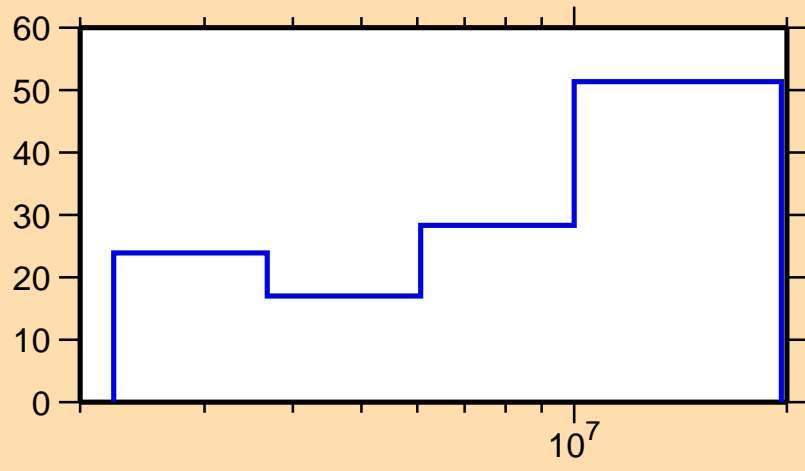
\Delta\sigma/\sigma vs. E for ^{200}\text{Pt}(n,n\text{cont.})
