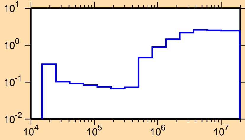
\sigma vs. E for ^{200}\text{Pt}(n,\text{nonel.})
