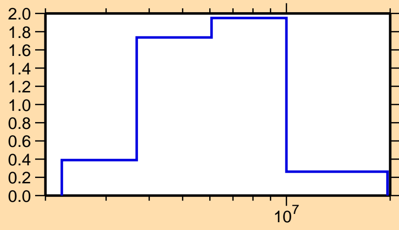
\sigma vs. E for ^{200}\text{Pt}(n,n\text{cont.})
