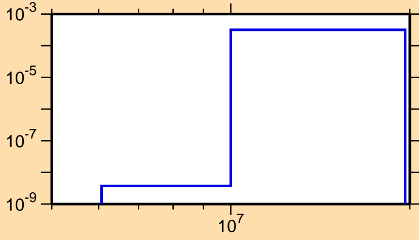
\sigma vs. E for ^{200}\text{Pt}(n,p)
