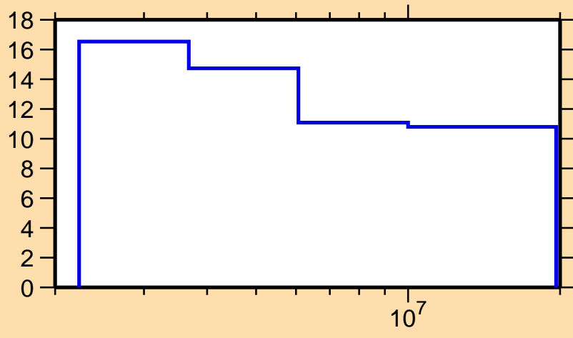
\Delta\sigma/\sigma vs. E for ^{200}\text{Pt}(n,n\text{onel.})
