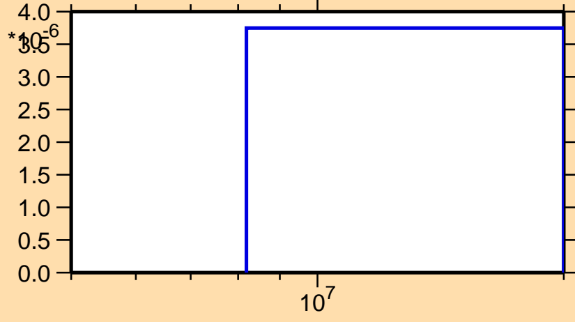
\sigma vs. E for ^{200}\text{Pt}(n,d)
