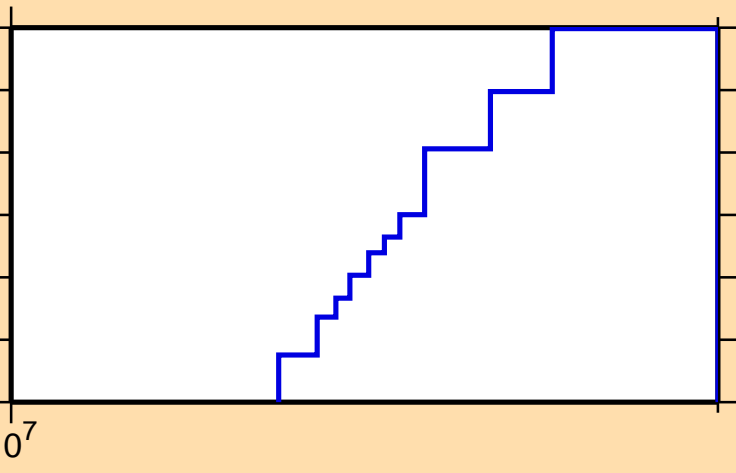
\sigma vs. E for ^{201}\text{Pt}(n,2n\alpha)
