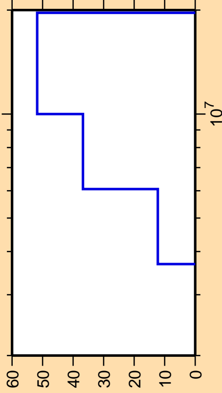
\Delta\sigma/\sigma vs. E for ^{201}\text{Pt}(n,n\text{cont.})
