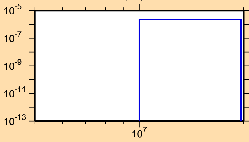
\sigma vs. E for ^{201}\text{Pt}(n,t)
