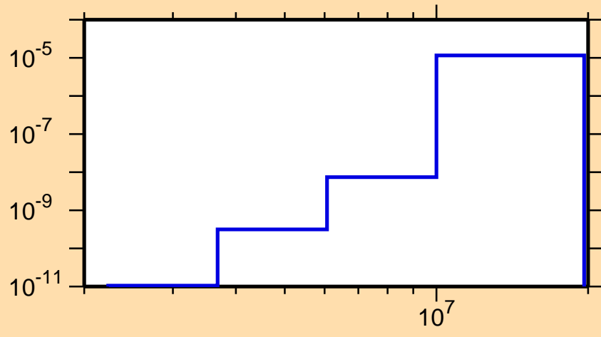
\sigma vs. E for ^{201}\text{Pt}(n,\alpha)
