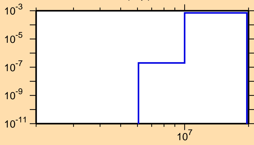
\sigma vs. E for ^{201}\text{Pt}(n,p)
