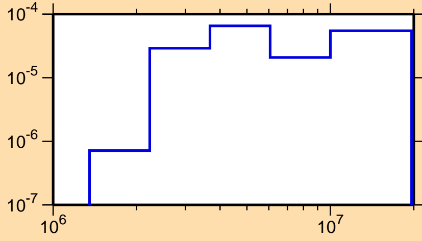
\sigma vs. E for ^{201}\text{Pt}(n,n_4)
