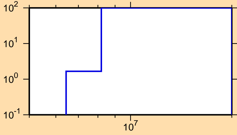
\Delta\sigma/\sigma vs. E for ^{202}\text{Pt}(n,p)
