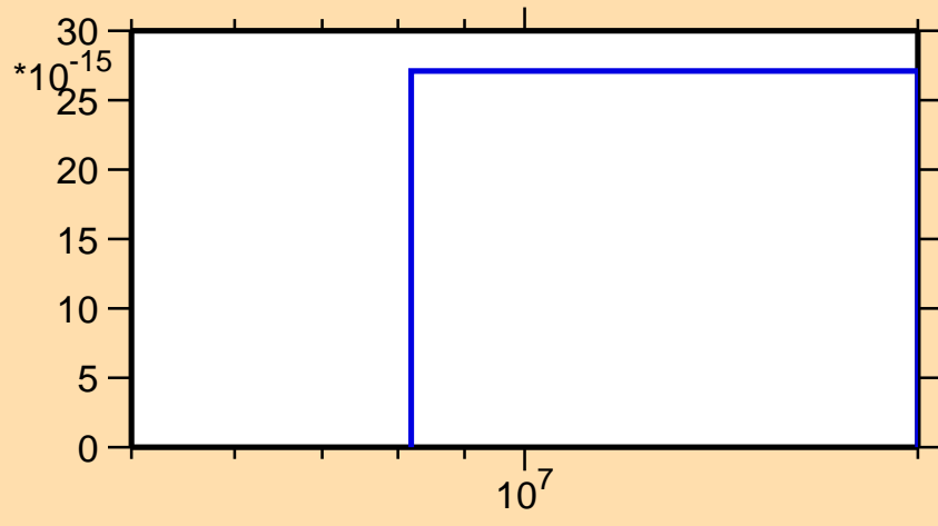
\sigma vs. E for ^{202}\text{Pt}(n,2np)
