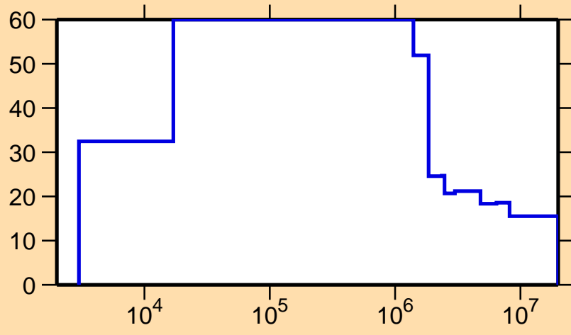
\Delta\sigma/\sigma vs. E for ^{202}\text{Pt}(n,\text{nonel.})
