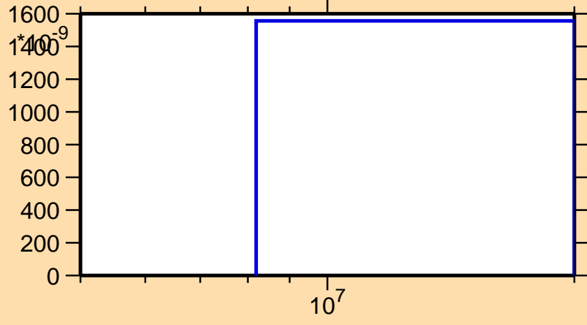
\sigma vs. E for ^{202}\text{Pt}(n,d)
