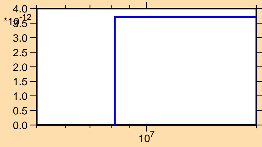
\sigma vs. E for ^{202}\text{Pt}(n,nt)
