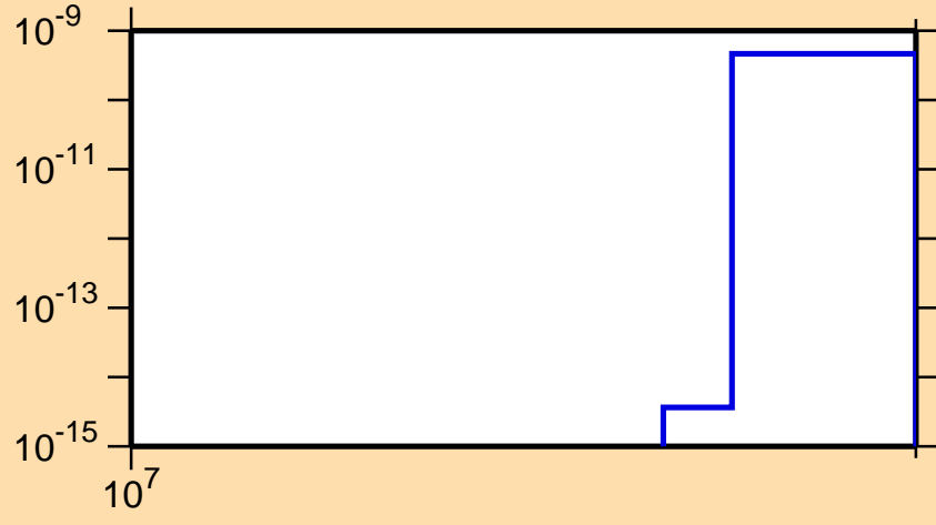
\sigma vs. E for ^{203}\text{Pt}(n,2np)
