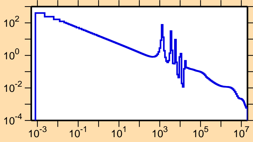
\sigma vs. E for ^{203}\text{Pt}(n,\gamma)
