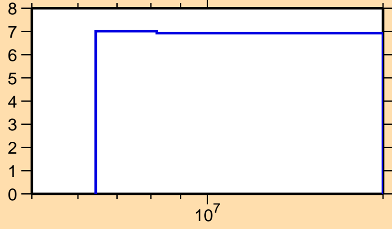
\Delta\sigma/\sigma vs. E for ^{203}\text{Pt}(n,\text{tot.})
