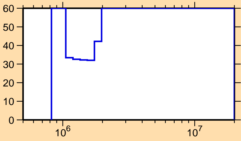
\Delta\sigma/\sigma vs. E for ^{204}\text{Pt}(n,n_1)
