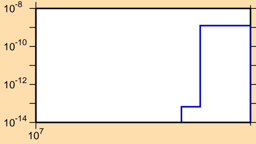
\sigma vs. E for ^{204}\text{Pt}(n,nt)
