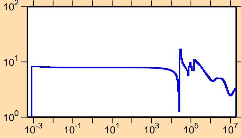
\sigma vs. E for ^{204}\text{Pt}(n,\text{el.})
