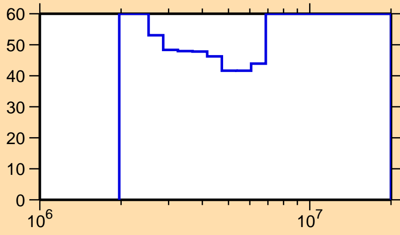
\Delta\sigma/\sigma vs. E for ^{204}\text{Pt}(n,n\text{cont.})
