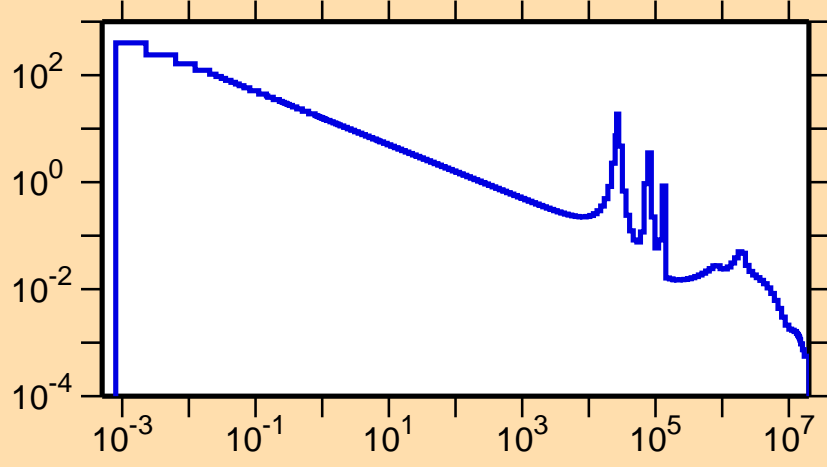
\sigma vs. E for ^{204}\text{Pt}(n,\gamma)
