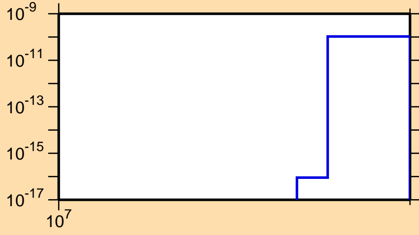
\sigma vs. E for ^{204}\text{Pt}(n,\text{nd})
