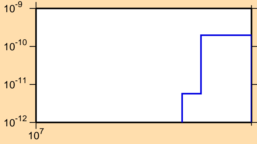
\sigma vs. E for ^{204}\text{Pt}(n,2n\alpha)
