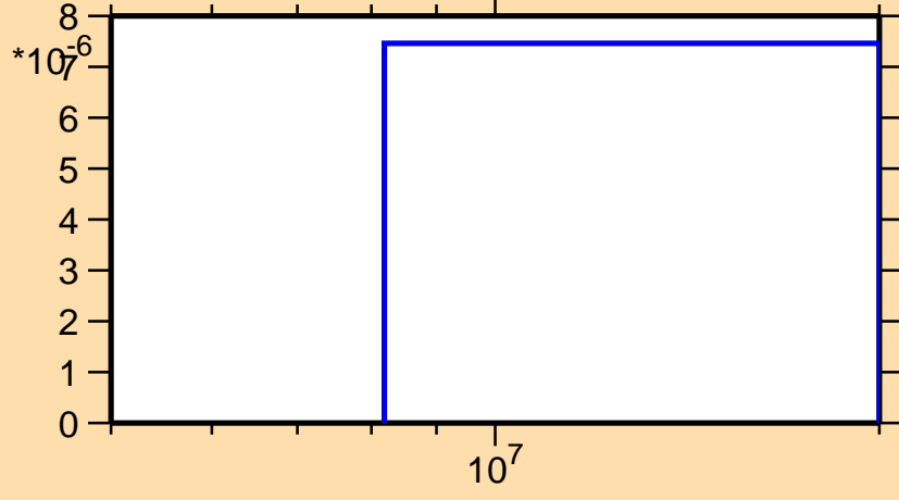
\sigma vs. E for ^{204}\text{Pt}(n,p)
