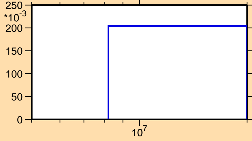
\sigma vs. E for ^{204}\text{Pt}(n,3n)
