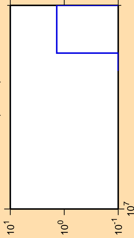
\Delta\sigma/\sigma vs. E for ^{205}\text{Pt}(n,3n\alpha)
