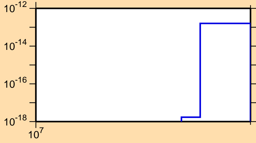
\sigma vs. E for ^{205}\text{Pt}(n,3n\alpha)
