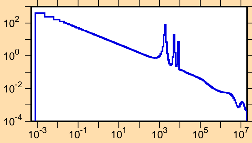
\sigma vs. E for ^{205}\text{Pt}(n,\gamma)
