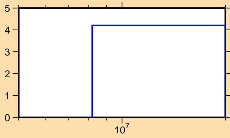
\Delta\sigma/\sigma vs. E for ^{205}\text{Pt}(n,\text{nonel.})
