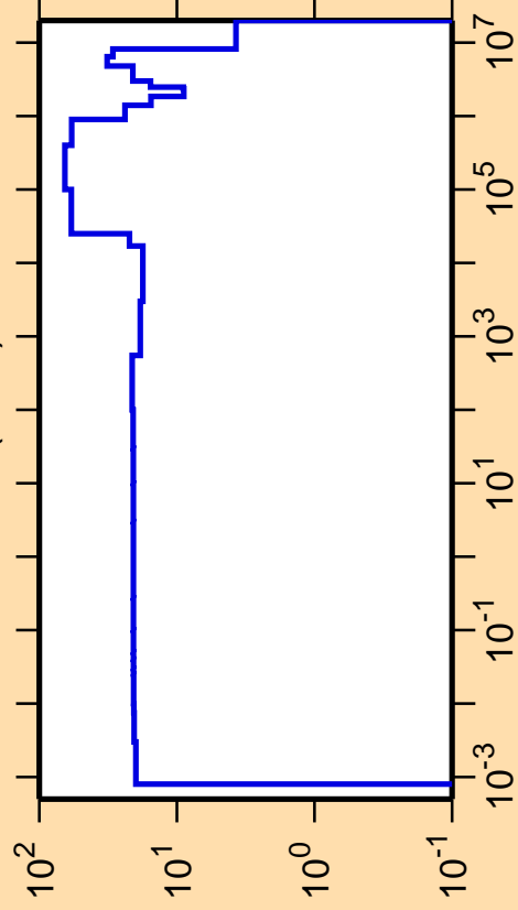
\Delta\sigma/\sigma vs. E for ^{205}\text{Pt}(n,\text{el.})
