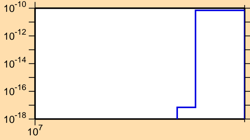
\sigma vs. E for ^{206}\text{Pt}(n,2np)
