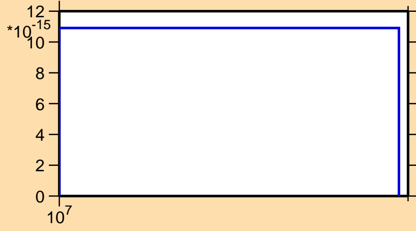
\sigma vs. E for ^{206}\text{Pt}(n,3n\alpha)
