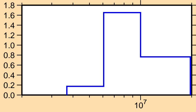
\sigma vs. E for ^{206}\text{Pt}(n,2n)
