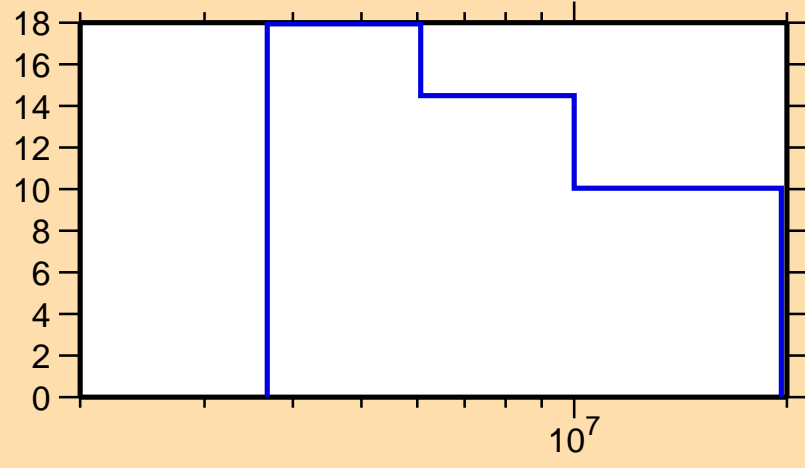
\Delta\sigma/\sigma vs. E for ^{206}\text{Pt}(n,\text{el.})
