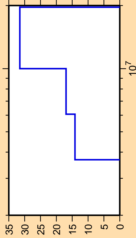
\Delta\sigma/\sigma vs. E for ^{206}\text{Pt}(n,2n)
