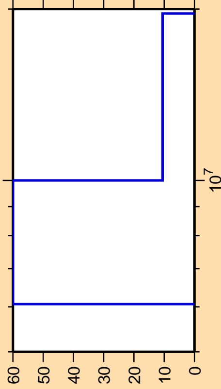
\Delta\sigma/\sigma vs. E for ^{206}\text{Pt}(n,3n)
