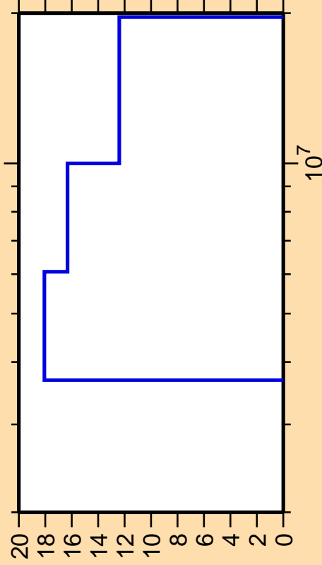
\Delta\sigma/\sigma vs. E for ^{206}\text{Pt}(n,n\text{cont.})
