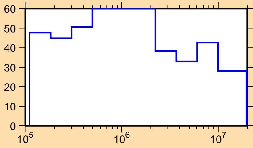
\Delta\sigma/\sigma vs. E for ^{206}\text{Pt}(n,n_1)
