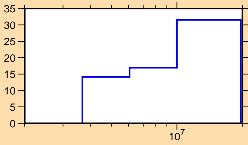
\Delta\sigma/\sigma vs. E for ^{206}\text{Pt}(n,2n)
