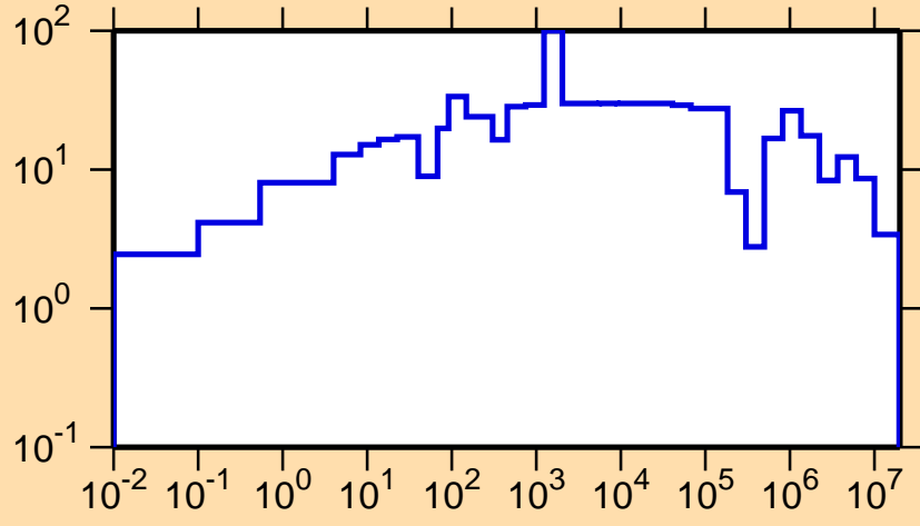
\Delta\sigma/\sigma vs. E for ^{206}\text{Pt}(n,\text{tot.})
