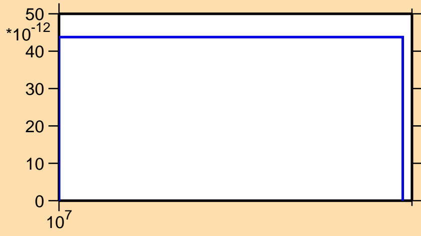
\sigma vs. E for ^{206}\text{Pt}(n,\text{nd})
