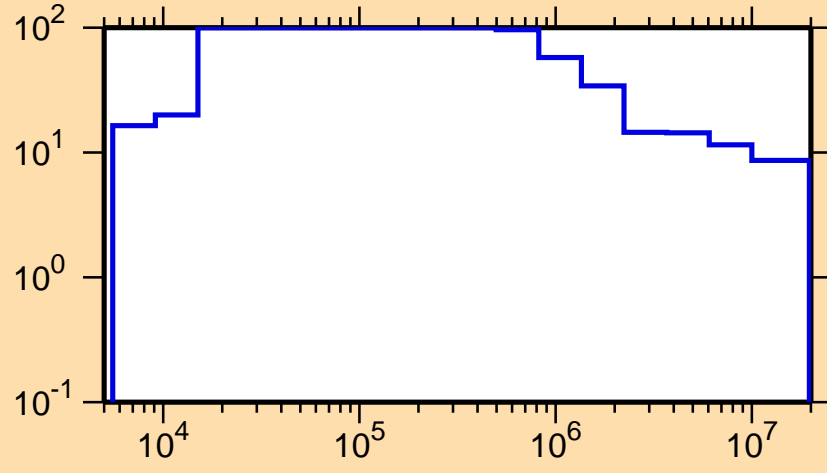
\Delta\sigma/\sigma vs. E for ^{206}\text{Pt}(n,\text{nonel.})
