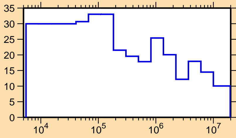
\Delta\sigma/\sigma vs. E for ^{206}\text{Pt}(n,\text{el.})
