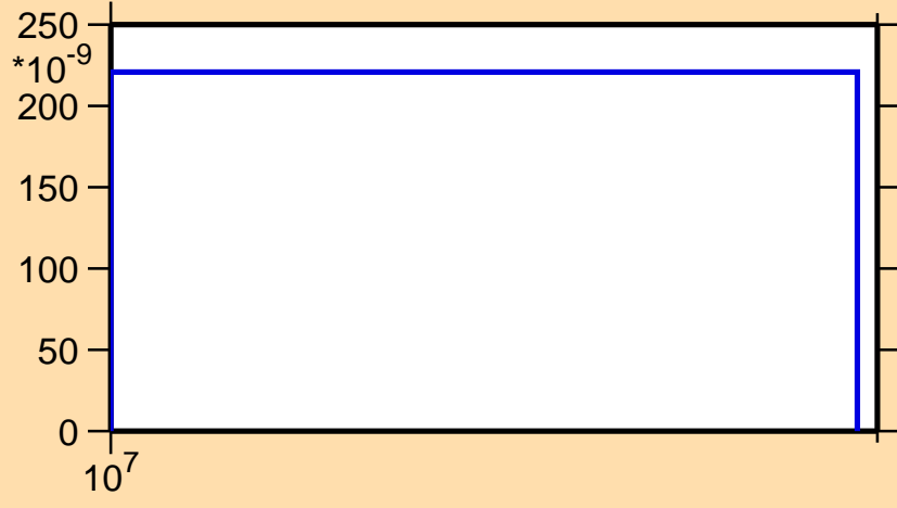
\sigma vs. E for ^{206}\text{Pt}(n,np)
