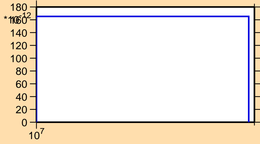
\sigma vs. E for ^{206}\text{Pt}(n,2n\alpha)
