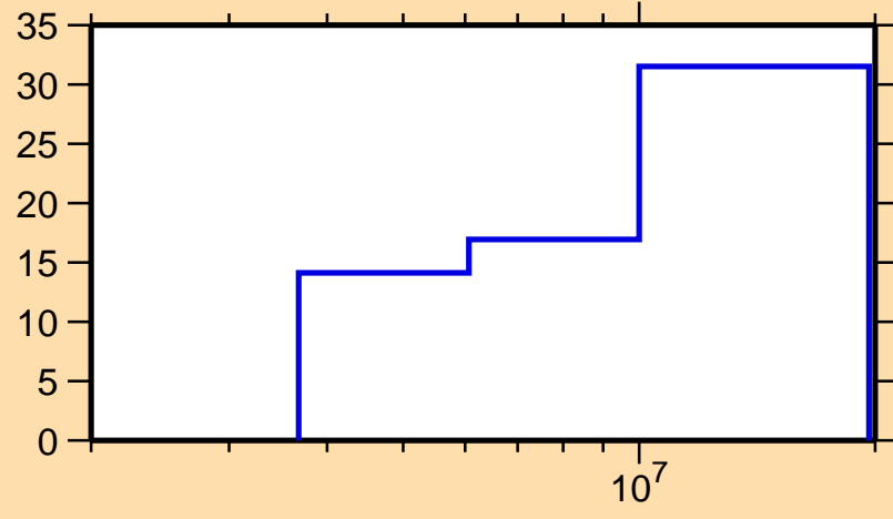
\Delta\sigma/\sigma vs. E for ^{206}\text{Pt}(n,2n)
