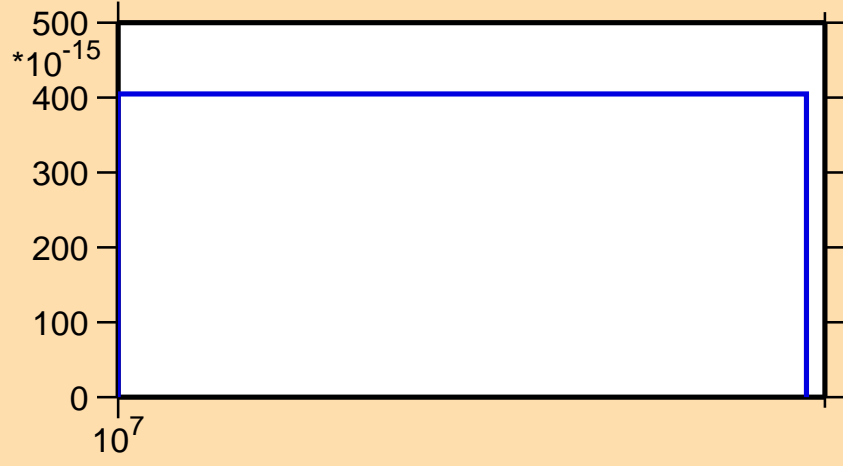
\sigma vs. E for ^{206}\text{Pt}(n,2np)
