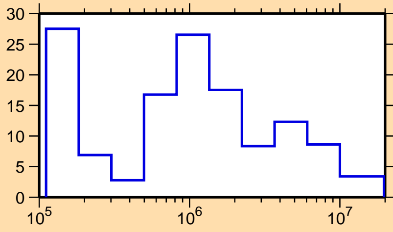
\Delta\sigma/\sigma vs. E for ^{206}\text{Pt}(n,\text{tot.})
