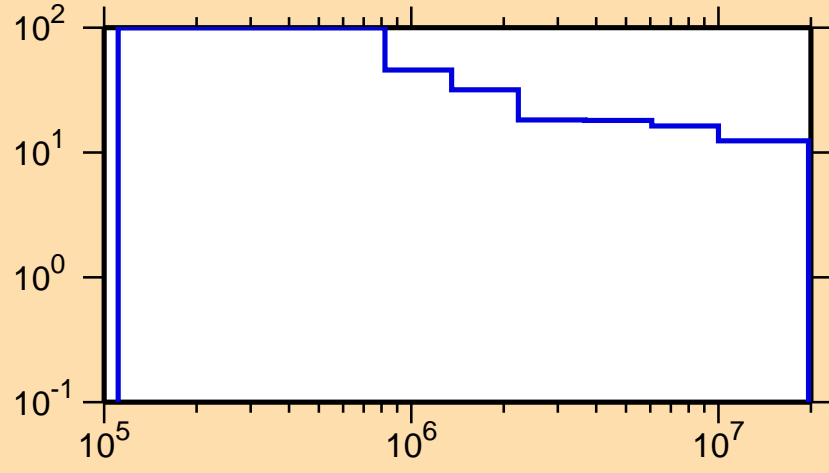
\Delta\sigma/\sigma vs. E for ^{206}\text{Pt}(n,n\text{cont.})
