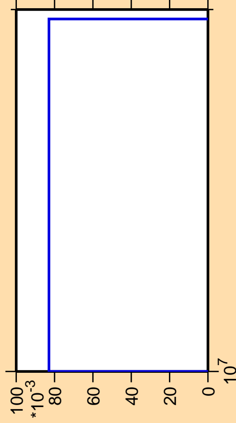
\Delta\sigma/\sigma vs. E for ^{206}\text{Pt}(n,3n\alpha)
