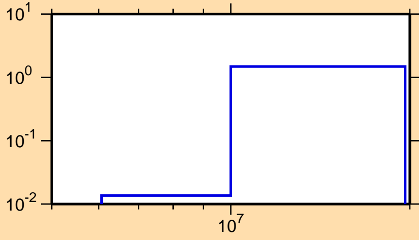
\sigma vs. E for ^{206}\text{Pt}(n,3n)
