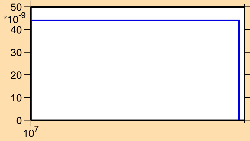
\sigma vs. E for ^{206}\text{Pt}(n,nt)
