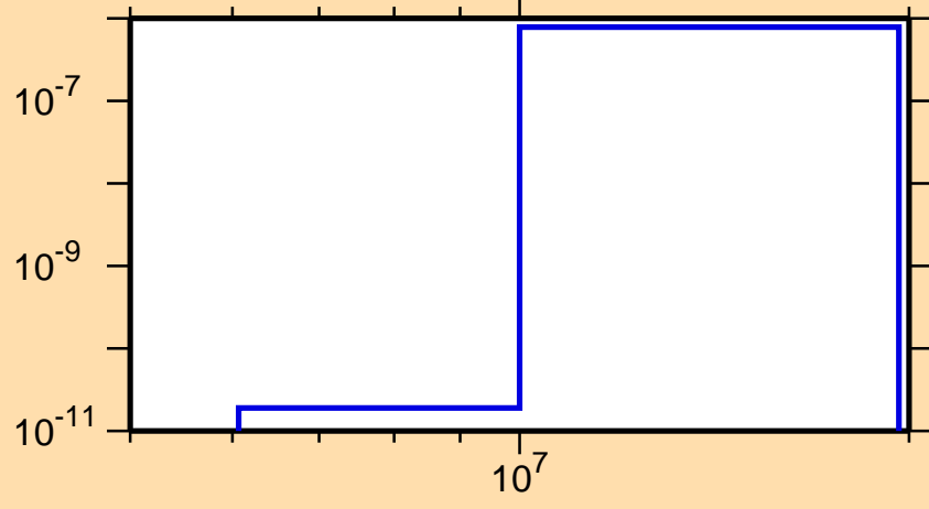
\sigma vs. E for ^{206}\text{Pt}(n,n\alpha)
