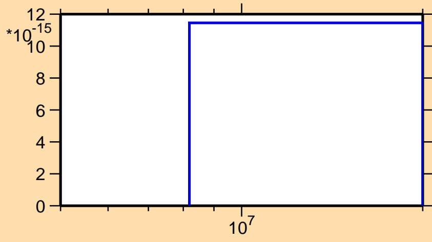
\sigma vs. E for ^{206}\text{Pt}(n,3n\alpha)
