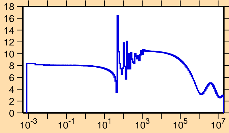
\sigma vs. E for ^{228}\text{Pu}(n,\text{el.})
