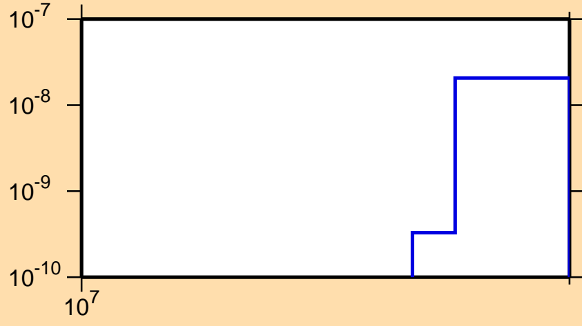
\sigma vs. E for ^{228}\text{Pu}(n,2np)
