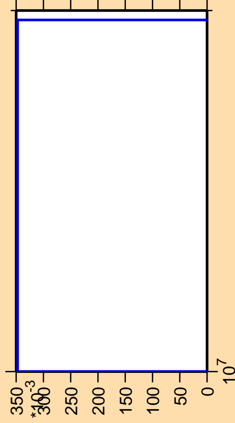
\Delta\sigma/\sigma vs. E for ^{228}\text{Pu}(n,\text{pd})
