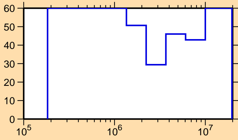
\Delta\sigma/\sigma vs. E for ^{228}\text{Pu}(n,n_1)
