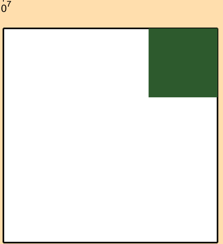
Correlation Matrix
