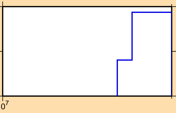
\sigma vs. E for ^{229}\text{Pu}(n,\text{pt})
