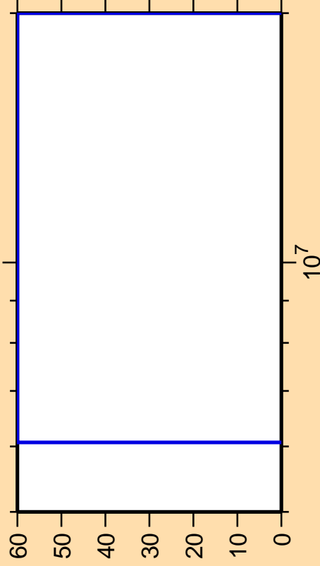
\Delta\sigma/\sigma vs. E for ^{229}\text{Pu}(n,n\text{cont.})
