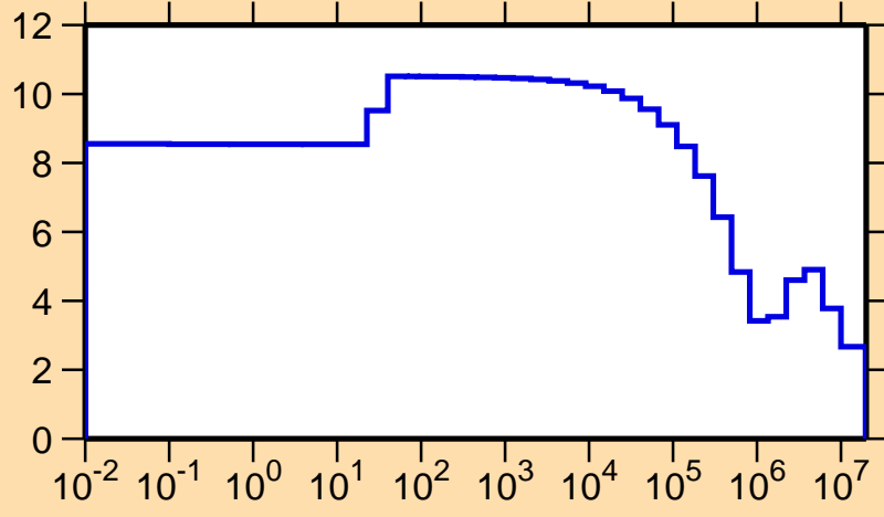
\sigma vs. E for ^{229}\text{Pu}(n,\text{el.})
