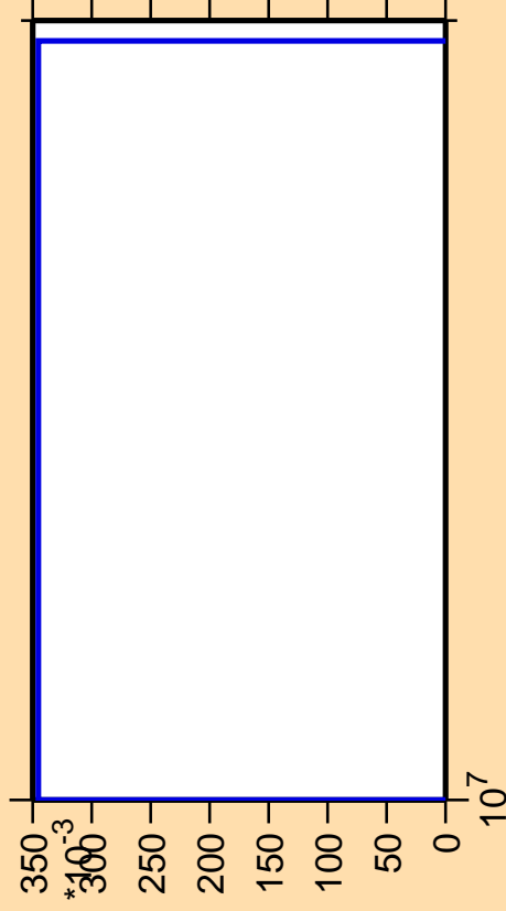
\Delta\sigma/\sigma vs. E for ^{229}\text{Pu} (mt 34)
