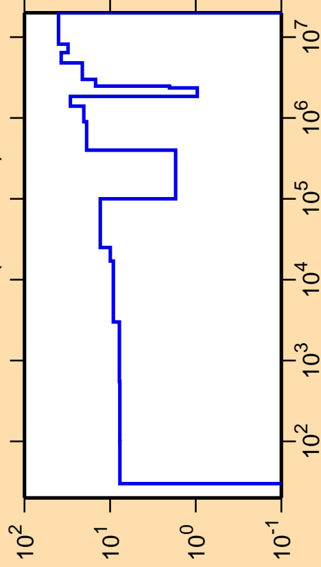
\Delta\sigma/\sigma vs. E for ^{229}\text{Pu}(n,\text{nonel.})
