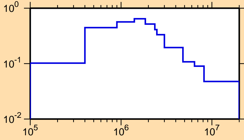
\sigma vs. E for ^{229}\text{Pu}(n,n_1)
