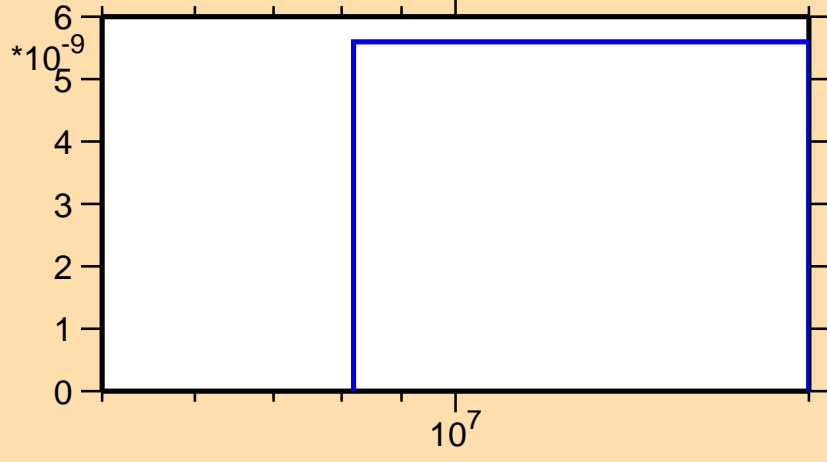
\sigma vs. E for ^{229}\text{Pu}(n,nd)
