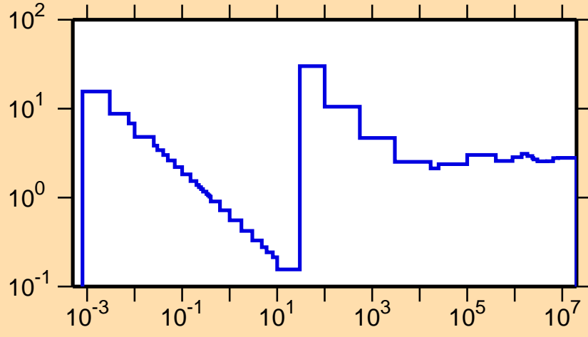
\sigma vs. E for ^{229}\text{Pu}(n,f)
