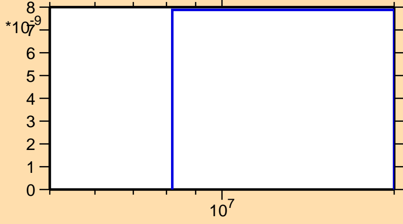
\sigma vs. E for ^{229}\text{Pu}(n,2np)
