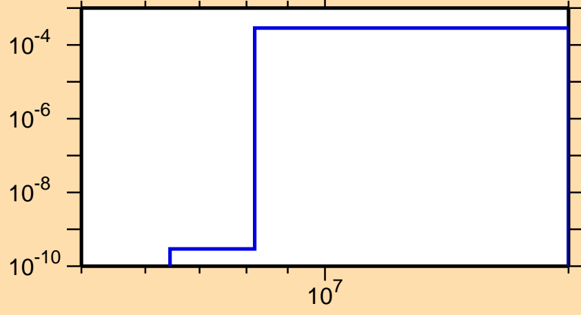
\sigma vs. E for ^{229}\text{Pu}(n,np)
