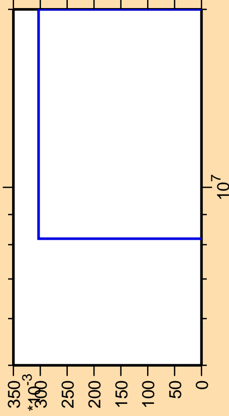
\Delta\sigma/\sigma vs. E for ^{229}\text{Pu}(\text{mt } 34)
