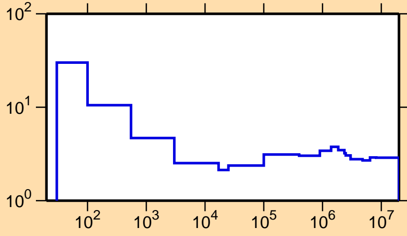
\sigma vs. E for ^{229}\text{Pu}(n,\text{nonel.})
