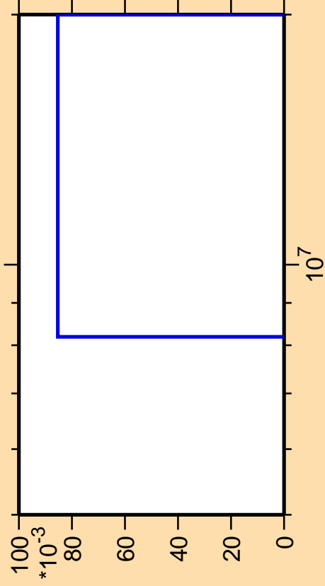
\Delta\sigma/\sigma vs. E for ^{229}\text{Pu}(n,\text{pt})
