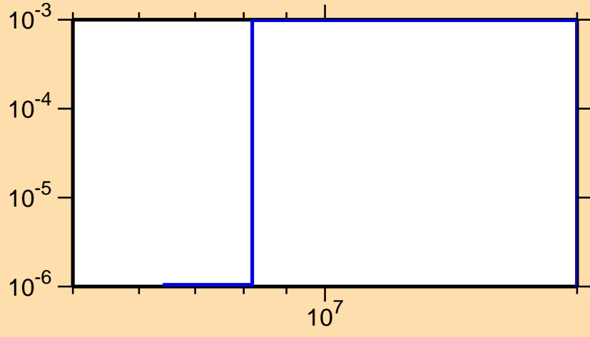
\sigma vs. E for ^{229}\text{Pu}(n,2n)
