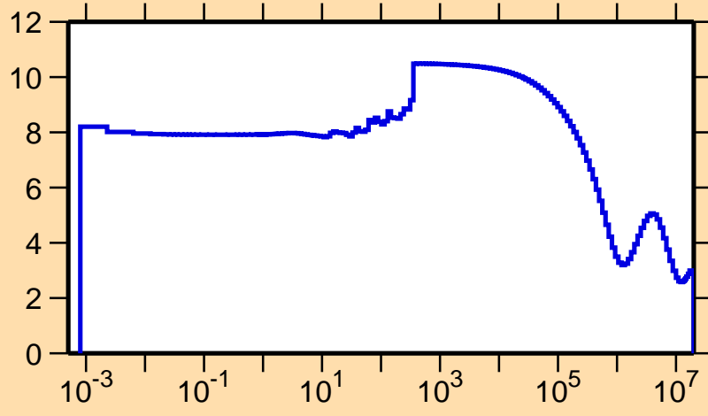
\sigma vs. E for ^{230}\text{Pu}(n,\text{el.})
