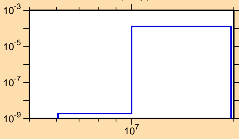
\sigma vs. E for ^{230}\text{Pu}(n,np)
