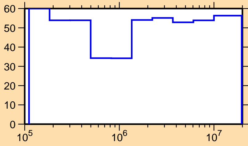
\Delta\sigma/\sigma vs. E for ^{230}\text{Pu}(n,n_1)
