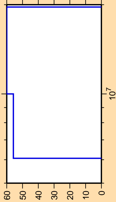
\Delta\sigma/\sigma vs. E for ^{230}\text{Pu}(n,np)
