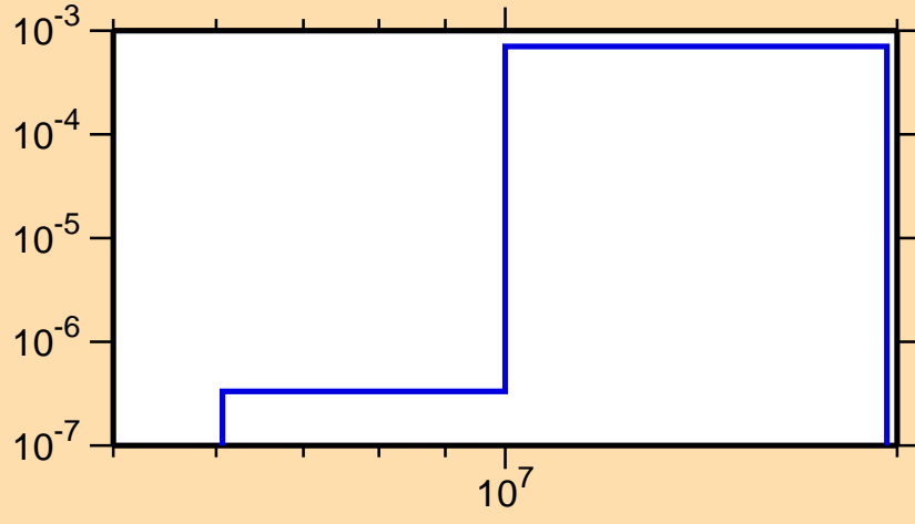
\sigma vs. E for ^{230}\text{Pu}(n,2n\alpha)
