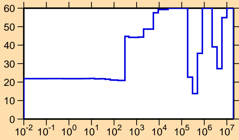
\Delta\sigma/\sigma vs. E for ^{230}\text{Pu}(n,el.)
