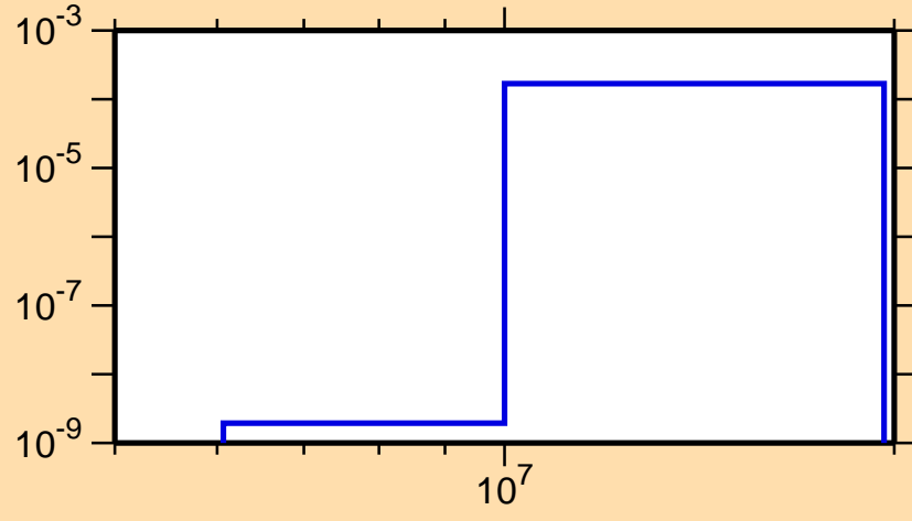
\sigma vs. E for ^{230}\text{Pu}(\text{mt117})
