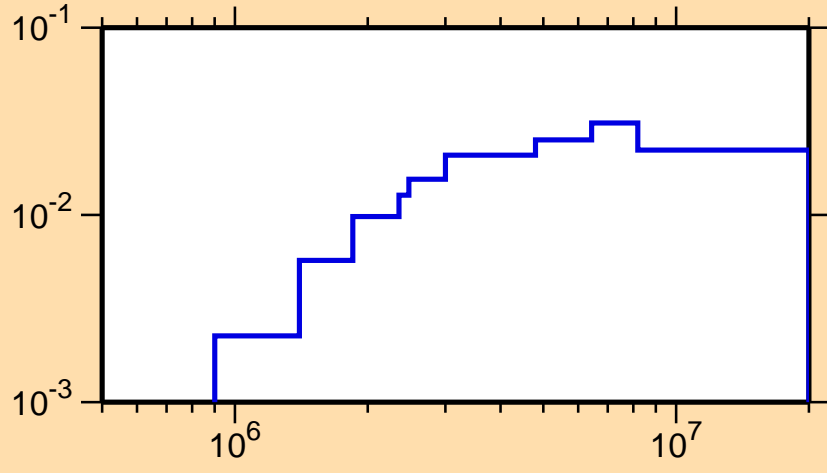
\sigma vs. E for ^{230}\text{Pu}(n,n\alpha)
