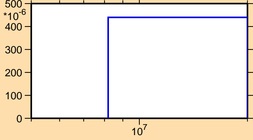
\sigma vs. E for ^{230}\text{Pu}(n,2n)
