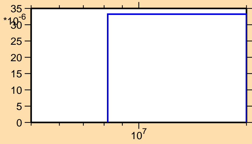
\sigma vs. E for ^{230}\text{Pu}(n,t)
