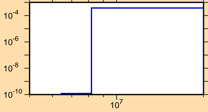
\sigma vs. E for ^{230}\text{Pu}(n,d)
