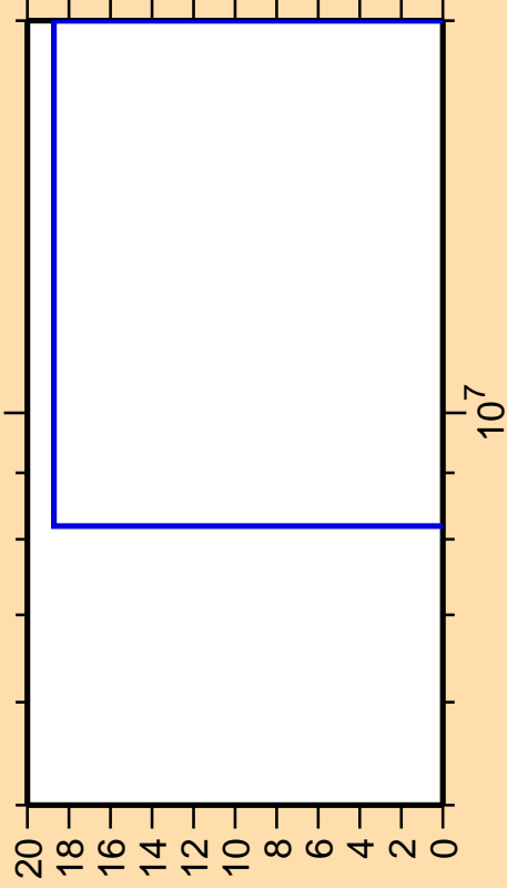
\Delta\sigma/\sigma vs. E for ^{230}\text{Pu}(n,f)
