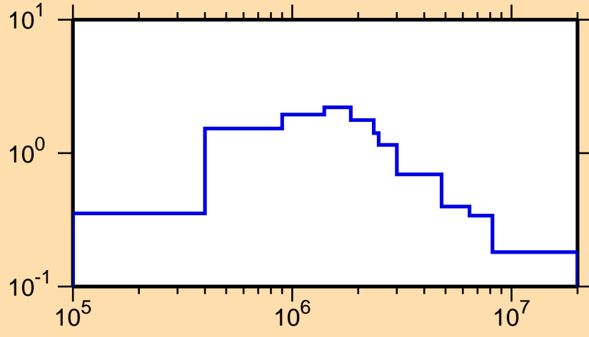
\sigma vs. E for ^{230}\text{Pu}(n,\text{inel.})
