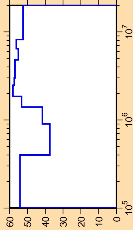
\Delta\sigma/\sigma vs. E for ^{230}\text{Pu}(n,\text{inel.})
