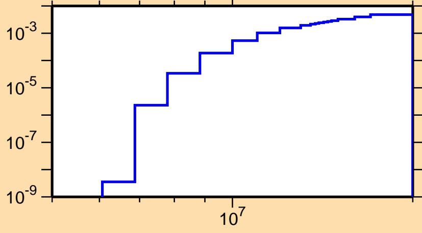
\sigma vs. E for ^{231}\text{Pu}(n,2n)
