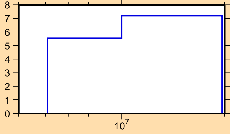
\Delta\sigma/\sigma vs. E for ^{231}\text{Pu}(n,\text{nonel.})
