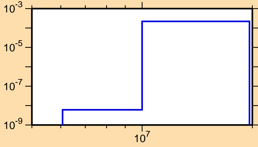
\sigma vs. E for ^{231}\text{Pu}(\text{mt117})
