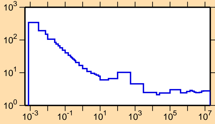
\sigma vs. E for ^{231}\text{Pu}(n,f)
