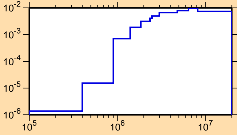
\sigma vs. E for ^{231}\text{Pu}(n,n\alpha)
