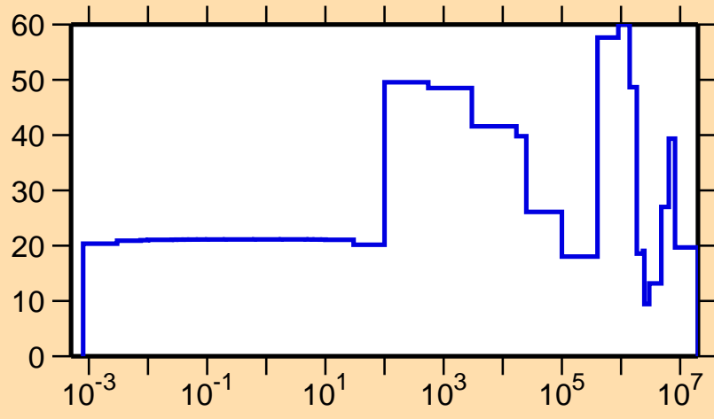
\Delta\sigma/\sigma vs. E for ^{231}\text{Pu}(n,el.)
