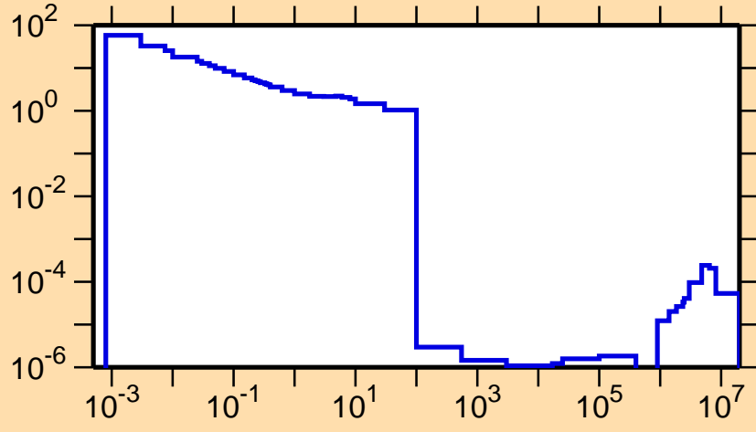
\sigma vs. E for ^{231}\text{Pu}(n,\gamma)
