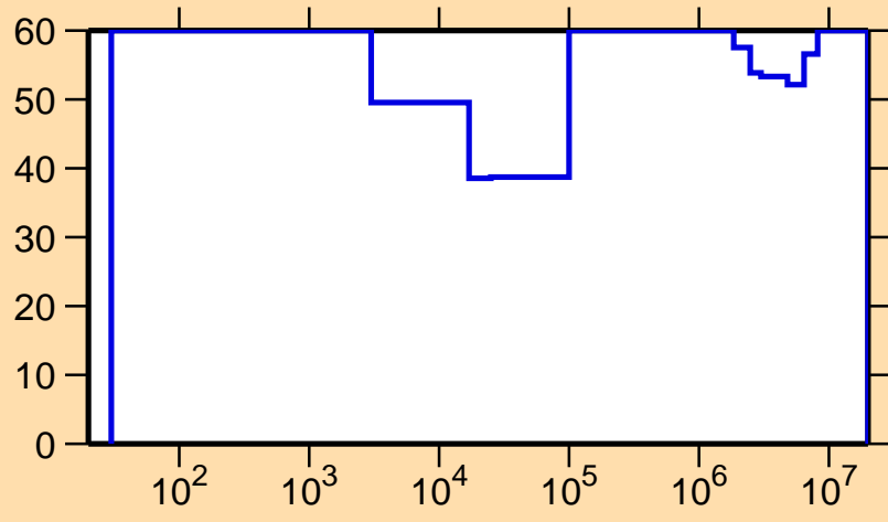
\Delta\sigma/\sigma vs. E for ^{231}\text{Pu}(n,p)
