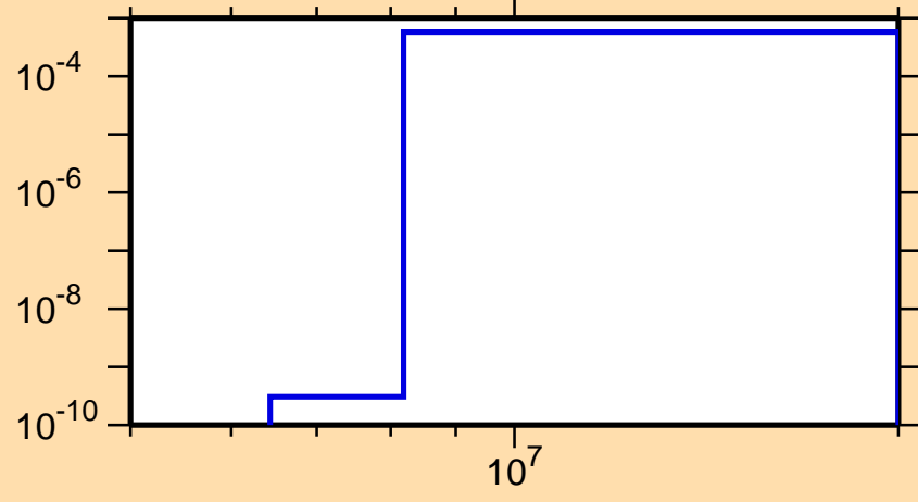
\sigma vs. E for ^{231}\text{Pu}(n,d)
