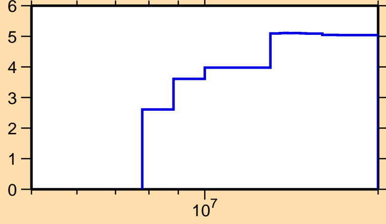
\Delta\sigma/\sigma vs. E for ^{232}\text{Pu}(n,\text{nonel.})
