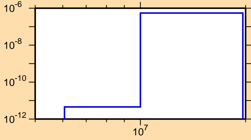
\sigma vs. E for ^{232}\text{Pu}(\text{mt117})
