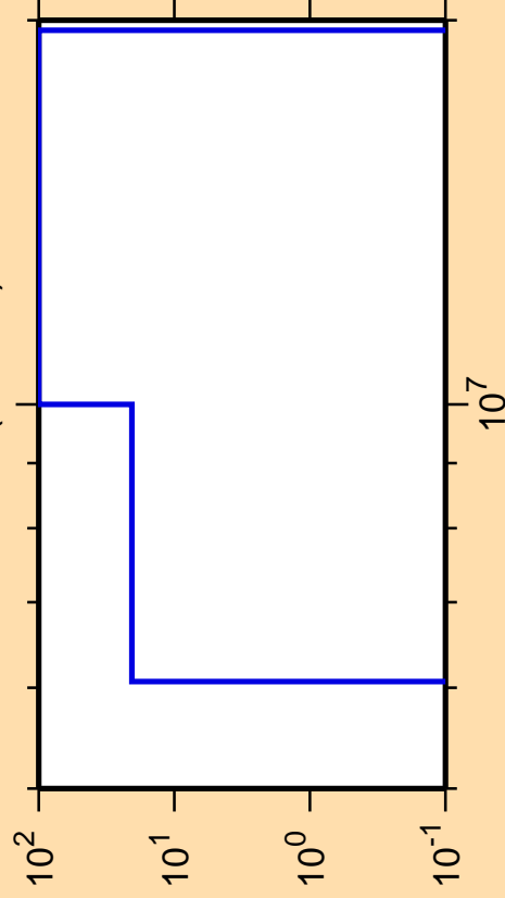
\Delta\sigma/\sigma vs. E for ^{232}\text{Pu}(\text{mt117})
