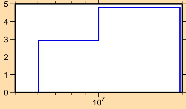
\Delta\sigma/\sigma vs. E for ^{232}\text{Pu}(n,\text{nonel.})
