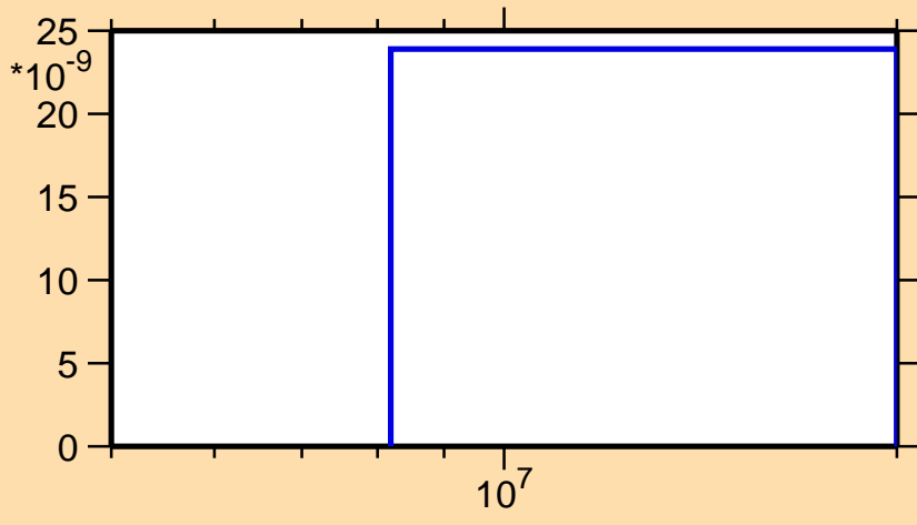
\sigma vs. E for ^{232}\text{Pu}(\text{mt } 45)
