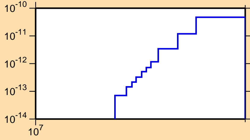
\sigma vs. E for ^{233}\text{Pu} (mt 45)
