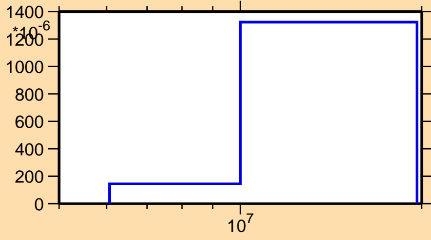
\sigma vs. E for ^{233}\text{Pu}(n,2n)
