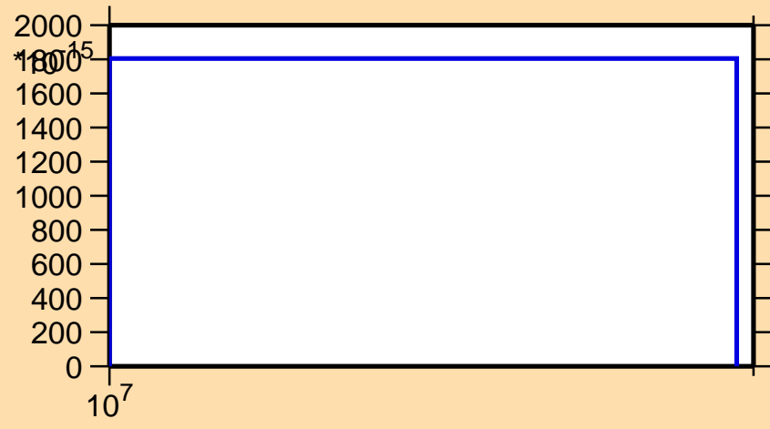
\sigma vs. E for ^{233}\text{Pu} (mt 45)
