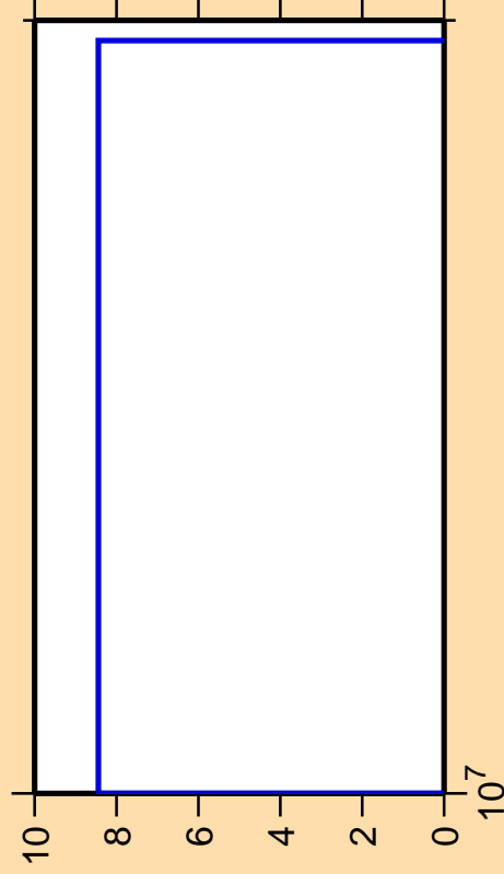
\Delta\sigma/\sigma vs. E for ^{233}\text{Pu} (mt 45)
