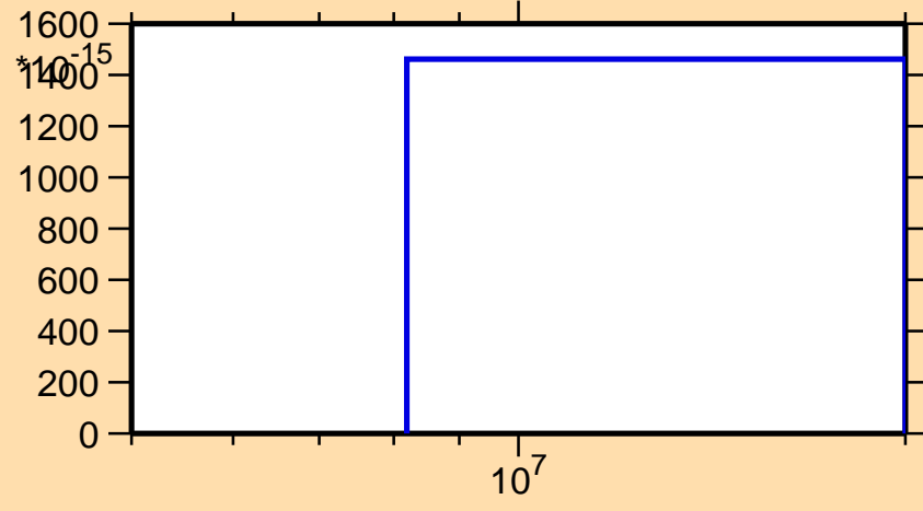
\sigma vs. E for ^{233}\text{Pu}(\text{mt 45})
