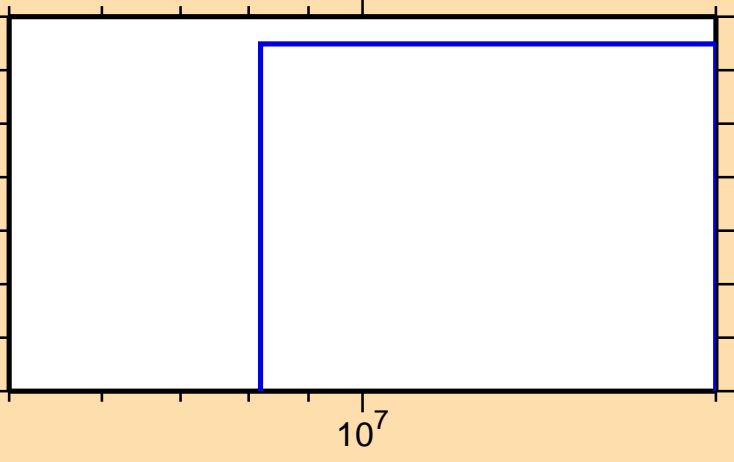
\sigma vs. E for ^{233}\text{Pu} (mt 34)
