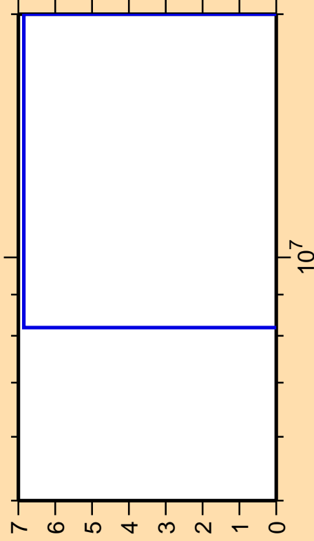
\Delta\sigma/\sigma vs. E for ^{233}\text{Pu}(\text{mt 45})
