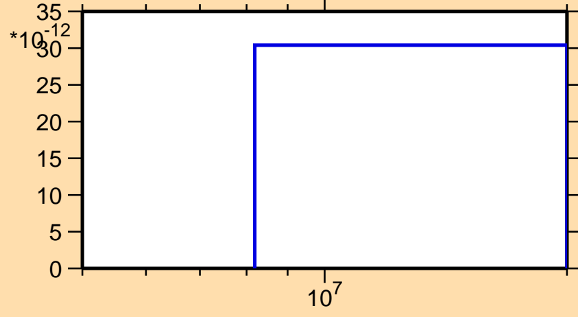
\sigma vs. E for ^{233}\text{Pu}(\text{mt117})
