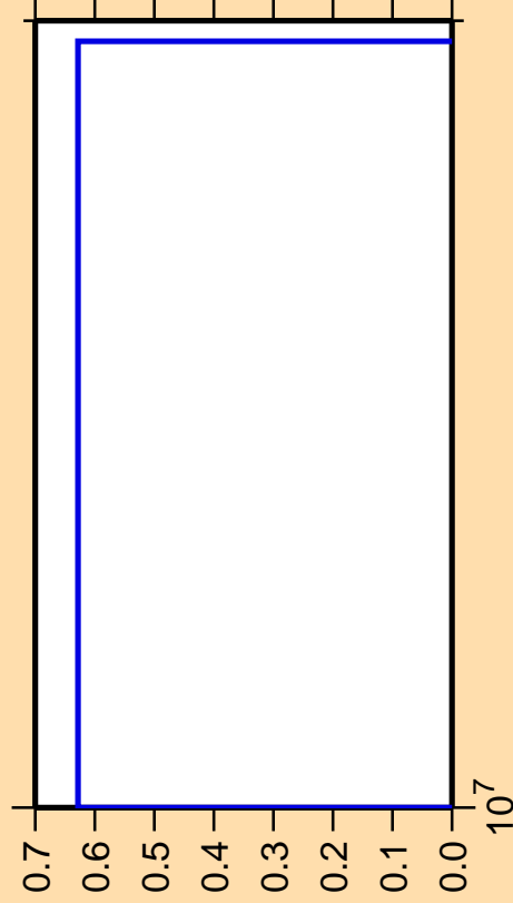
\Delta\sigma/\sigma vs. E for ^{234}\text{Pu} (mt 45)
