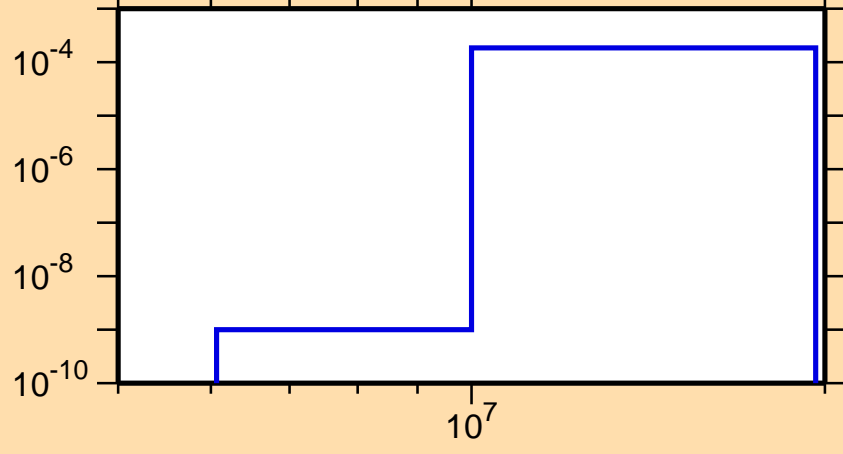
\sigma vs. E for ^{234}\text{Pu}(n,d)
