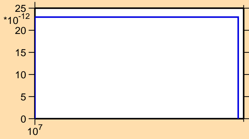
\sigma vs. E for ^{234}\text{Pu}(\text{mt117})
