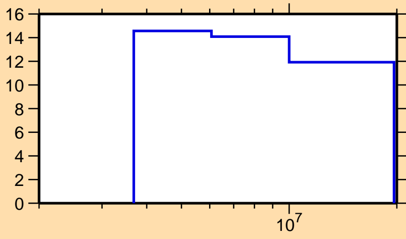
\Delta\sigma/\sigma vs. E for ^{234}\text{Pu}(n,f)
