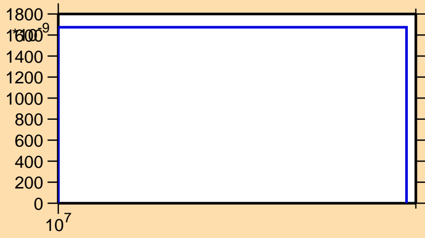
\sigma vs. E for ^{234}\text{Pu}(n,3n\alpha)
