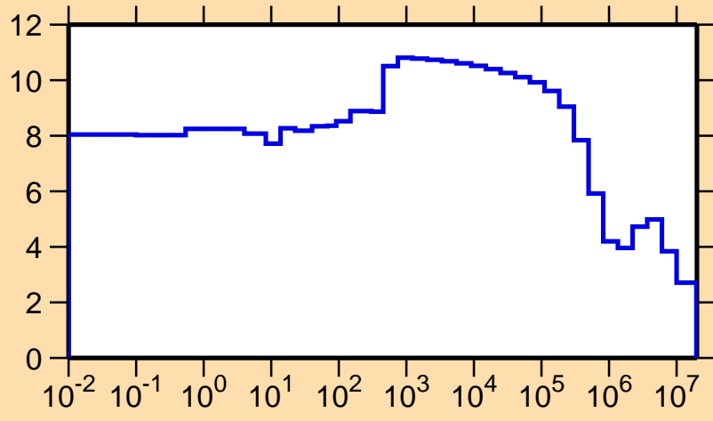
\sigma vs. E for ^{234}\text{Pu}(n,\text{el.})
