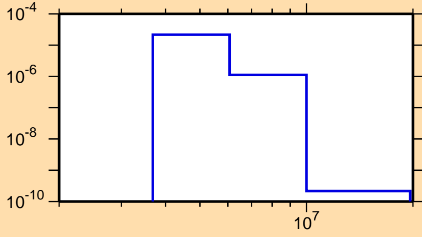
\sigma vs. E for ^{234}\text{Pu}(n,n_1)
