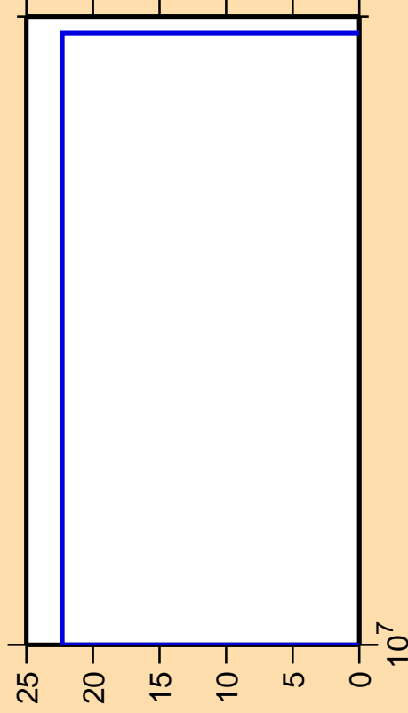
\Delta\sigma/\sigma vs. E for ^{234}\text{Pu}(\text{mt117})
