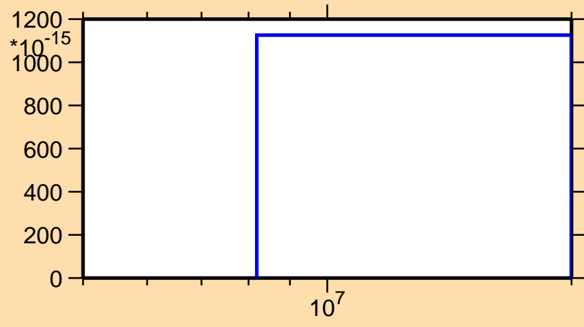
\sigma vs. E for ^{234}\text{Pu}(\text{mt } 45)
