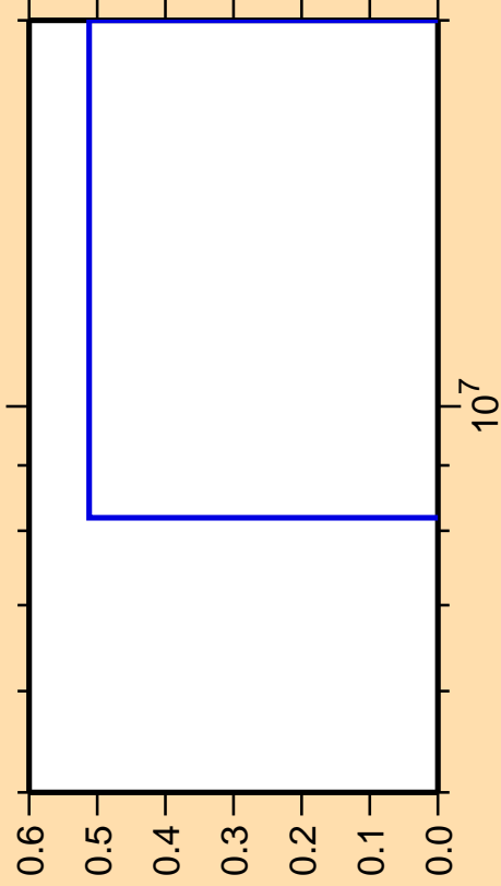
\Delta\sigma/\sigma vs. E for ^{234}\text{Pu}(\text{mt } 45)
