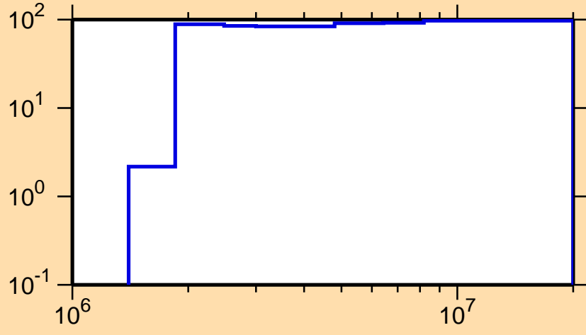
\Delta\sigma/\sigma vs. E for ^{234}\text{Pu}(n,p)
