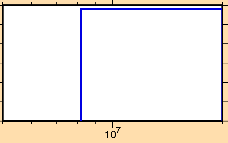
\sigma vs. E for ^{234}\text{Pu}(n,p\alpha)
