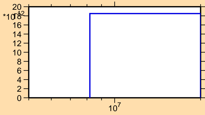
\sigma vs. E for ^{234}\text{Pu}(\text{mt117})
