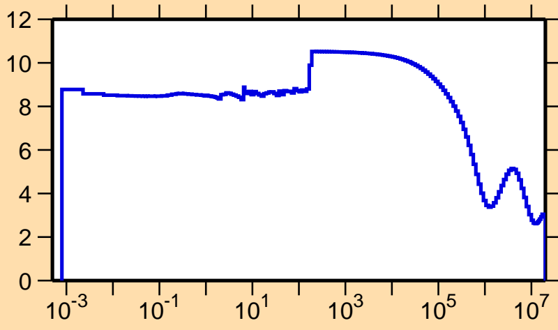
\sigma vs. E for ^{235}\text{Pu}(n,\text{el.})
