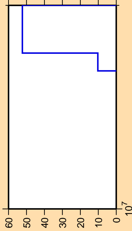
\Delta\sigma/\sigma vs. E for ^{235}\text{Pu} (mt 45)
