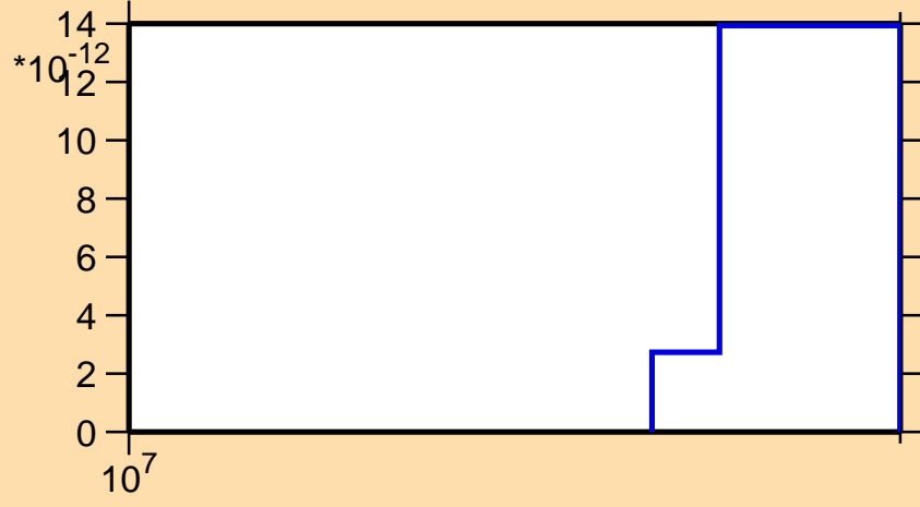
\sigma vs. E for ^{235}\text{Pu} (mt 45)
